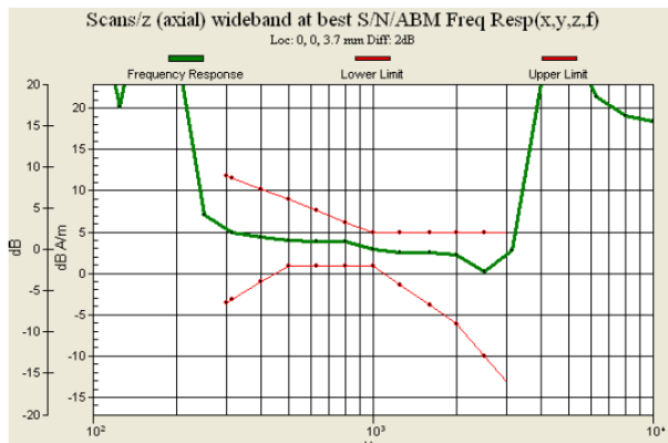
Fig. 9.7 GSM1900 Ch810 (DUT with Keypad 1)
