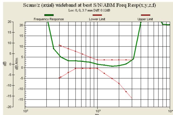
Fig. 9.14 WCDMA Band IV Ch1413 (DUT with Keypad 1)
