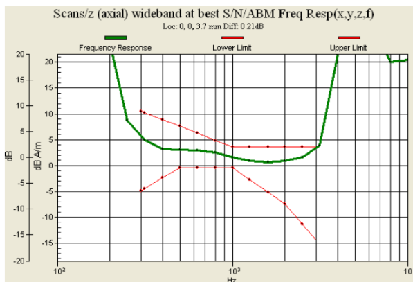
Fig. 9.16 WCDMA Band IV Ch1312 (DUT with Keypad 2)
