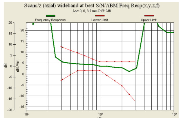
Fig. 9.2 GSM850 Ch189 (DUT with Keypad 1)
