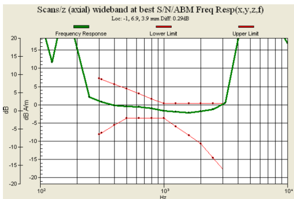
Fig. 9.17 WCDMA Band II Ch9262 (DUT with Keypad 1)
