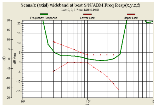
Fig. 9.10 WCDMA Band V Ch4182 (DUT with Keypad 1))
