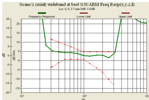
Fig. 9.1 GSM850 Ch128 (DUT with Keypad 1)
