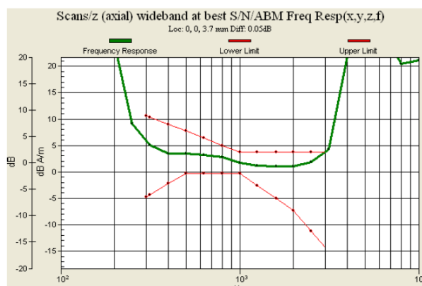
Fig. 9.12 WCDMA Band V Ch4182 (DUT with Keypad 2)
