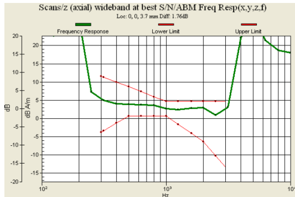
Fig. 9.8 GSM1900 Ch810 (DUT with Keypad 2)
