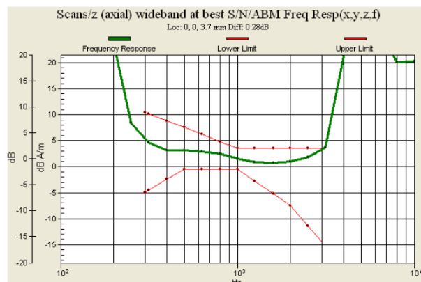
Fig. 9.20 WCDMA Band II Ch9538 (DUT with Keypad 2)
