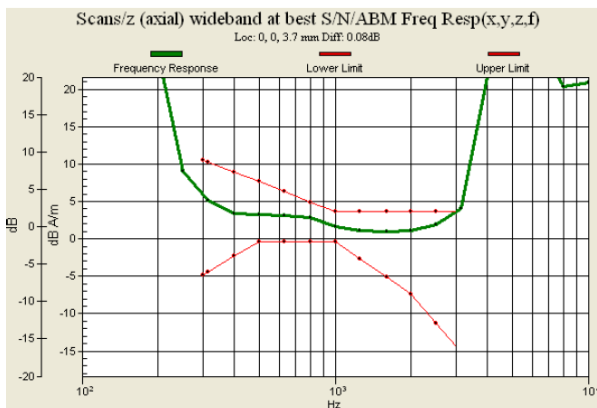
Fig. 9.18 WCDMA Band II Ch9400 (DUT with Keypad 1)
