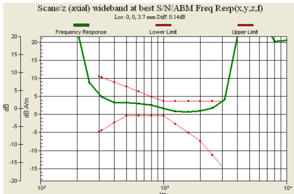
Fig. 9.13 WCDMA Band IV Ch1312 (DUT with Keypad 1)
