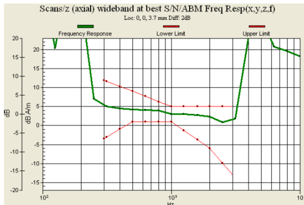
Fig. 9.3 GSM850 Ch251 (DUT with Keypad 1)
