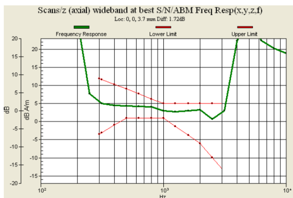
Fig. 9.5 GSM1900 Ch512 (DUT with Keypad 1)
