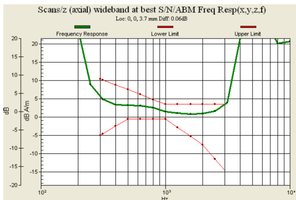
Fig. 9.15 WCDMA Band IV Ch1513 (DUT with Keypad 1)
