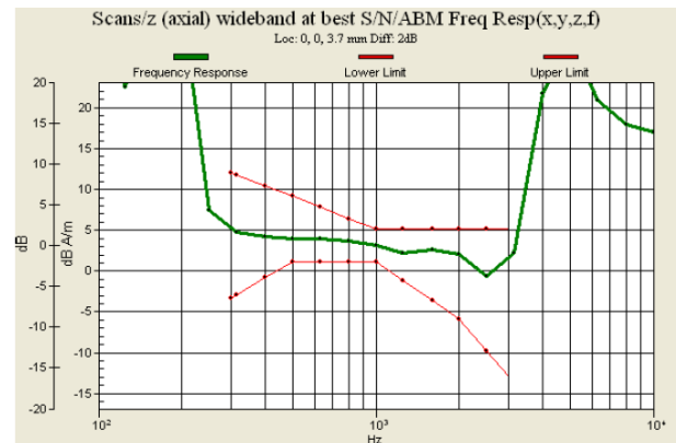
Fig. 9.4 GSM850 Ch251 (DUT with Keypad 2)
