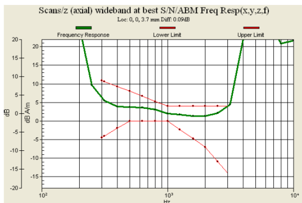
Fig. 9.9 WCDMA Band V Ch4132 (DUT with Keypad 1))
