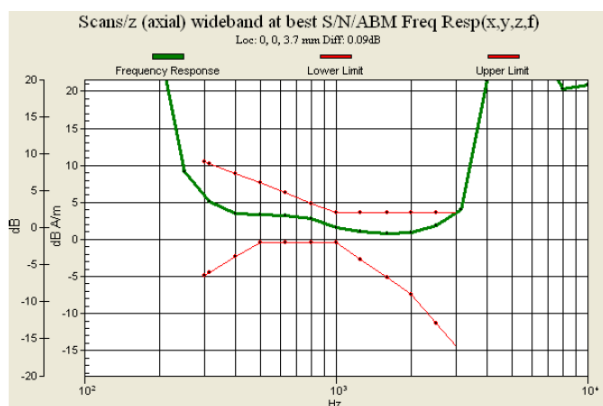
Fig. 9.19 WCDMA Band II Ch9538 (DUT with Keypad 1)
