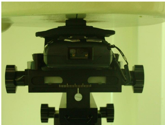
Back of the DUT and Holster with Phantom 0 cm Gap
