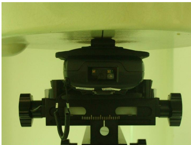
Front of the DUT and Holster with Phantom 0 cm Gap
