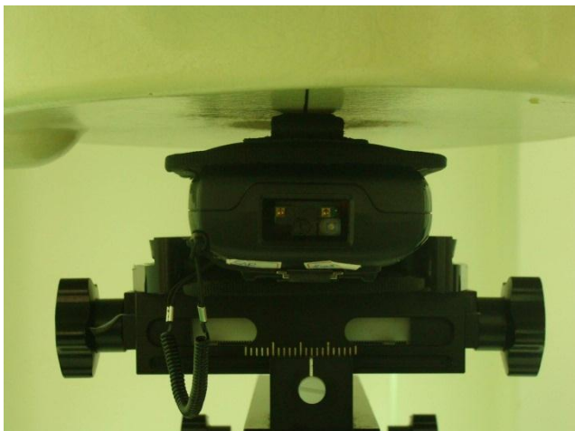
Front of the DUT and Holster with Phantom 0 cm Gap
