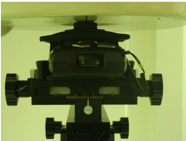
Back of the DUT and Holster with Phantom 0 cm Gap
