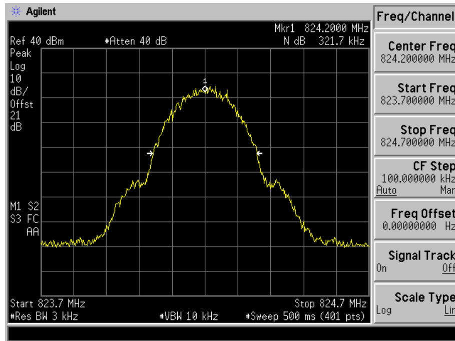
GSM 850 - Circuit Switched (GSM Mode CH 128)
