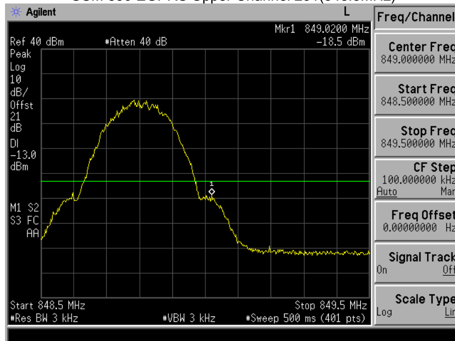
GSM 850 EGPRS Upper Channel 251(848.8MHz)
