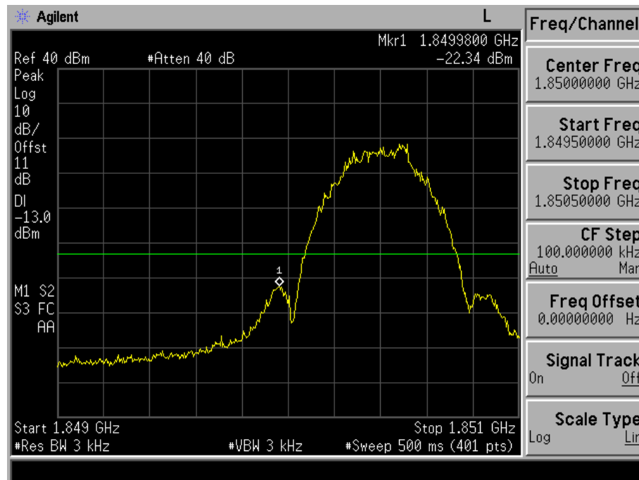
PCS 1900 EGPRS Lower Channel 512 (1850.2MHz)
