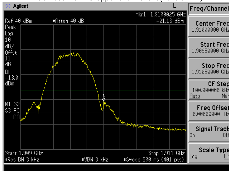
PCS 1900 EGPRS Upper Channel 810(1910.0MHz)
