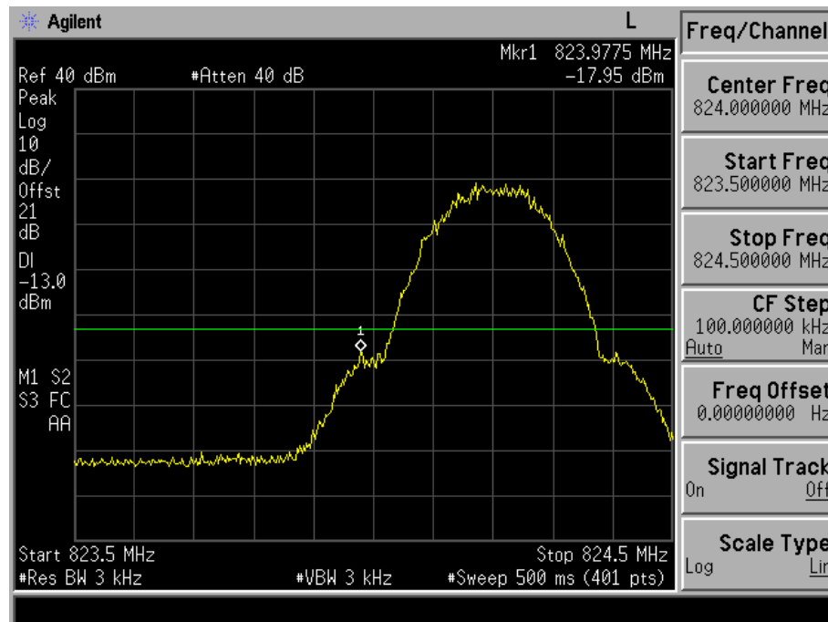
GSM 850 EGPRS Lower Channel 128 (824.2MHz)
