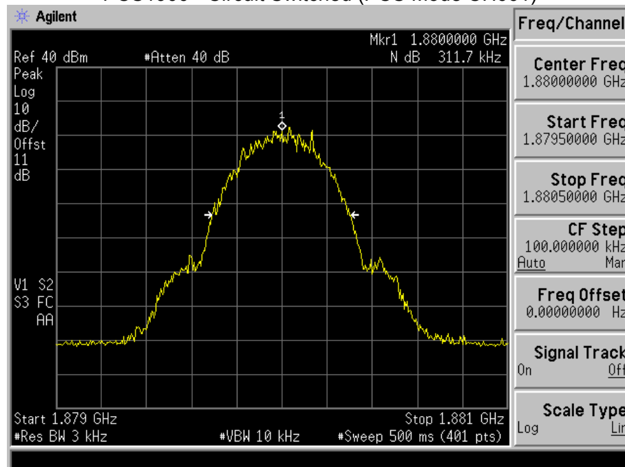
PCS1900 - Circuit Switched (PCS Mode CH661)
