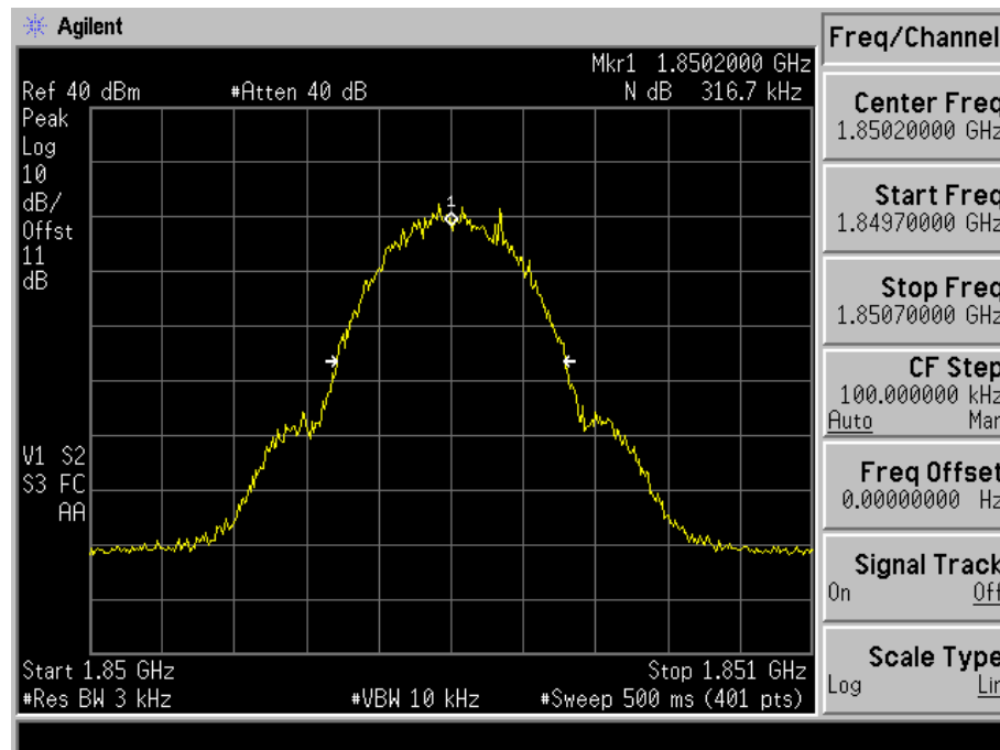
PCS1900 - Circuit Switched (PCS Mode CH 512)
