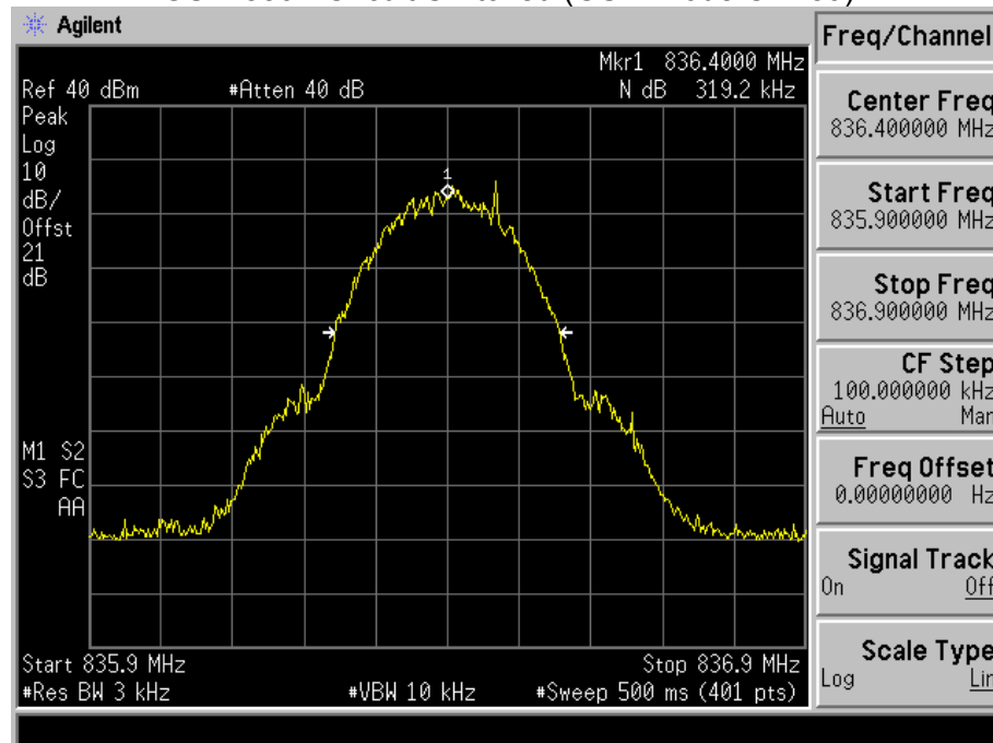
GSM 850 - Circuit Switched (GSM Mode CH189)
