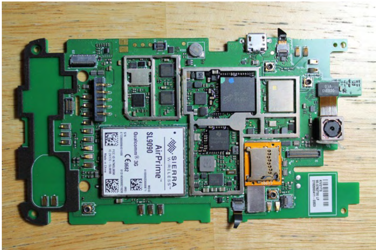
Brand Name: Honeywell Model Name: 70ELGN Main board with shields removed (Top view)
