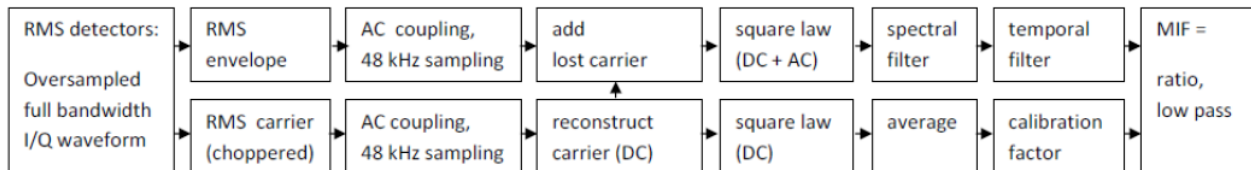
Figure 39.2: Block diagram for measuring or simulating MIF from modulated waveforms
