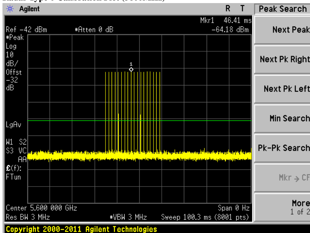
Radar Type 0 Calibration Plot (5600MHz)
