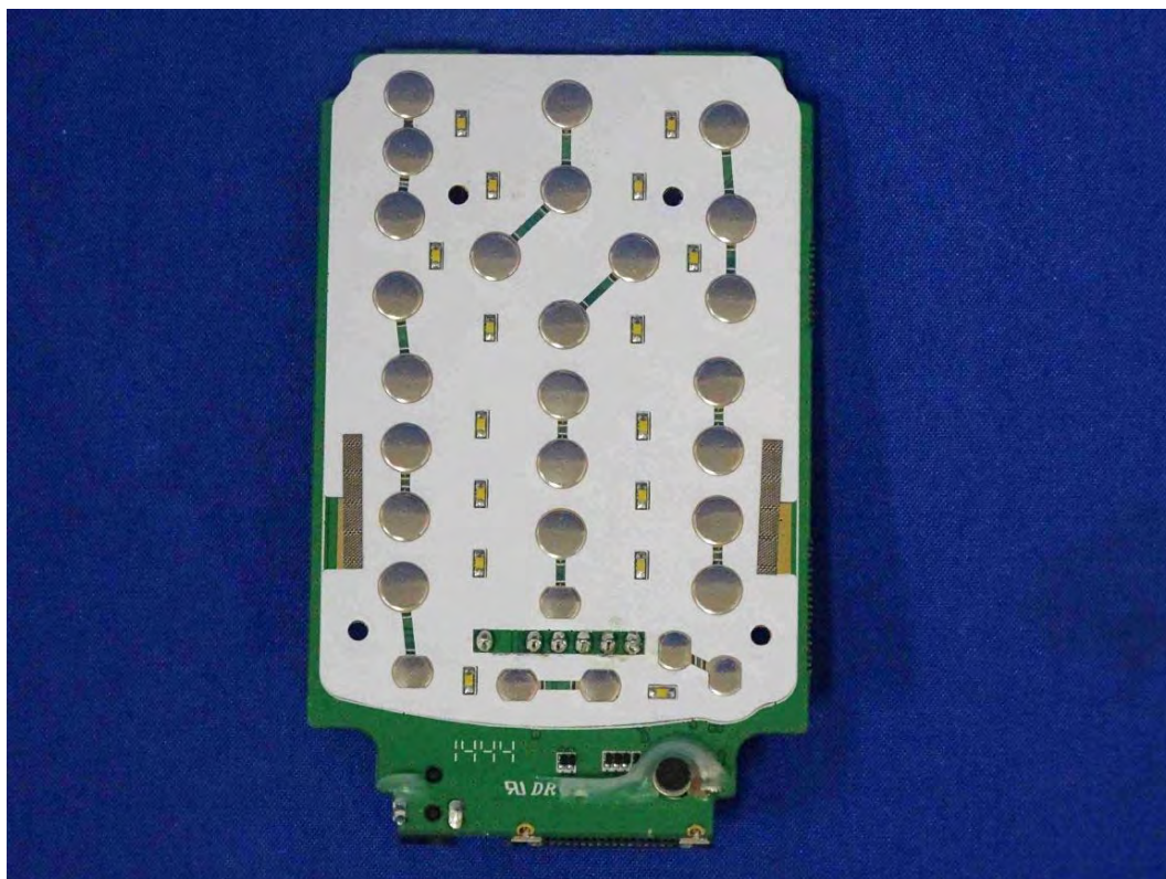
(43) EUT Photo
