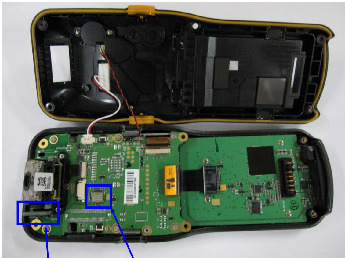
Bluetooth Antenna
