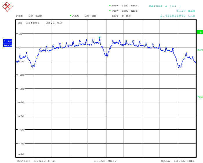
PSD 100kHz Plot on 802.11b Channel 01
