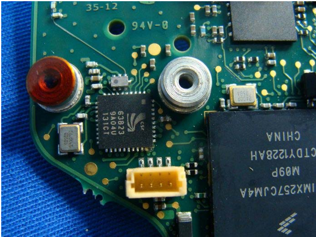
(14) EUT Photo (Bluetooth Chipset)
