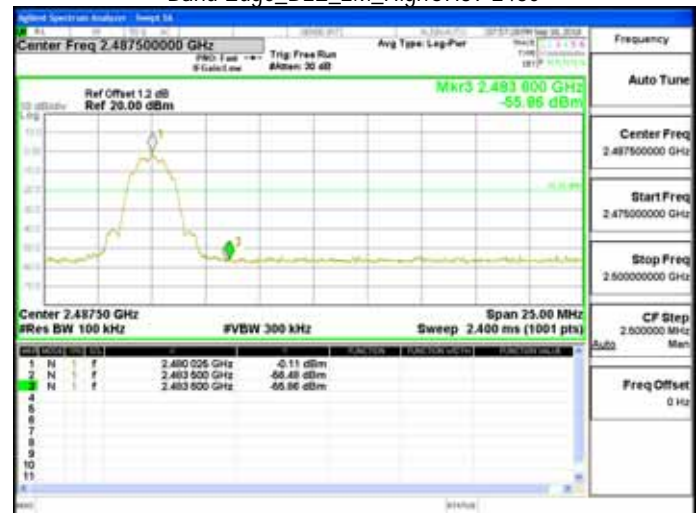
Band Edge_BLE_2M_HighCH39-2480
