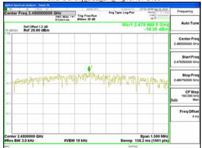
Power Density_BLE_2M_HighCH39-2480
