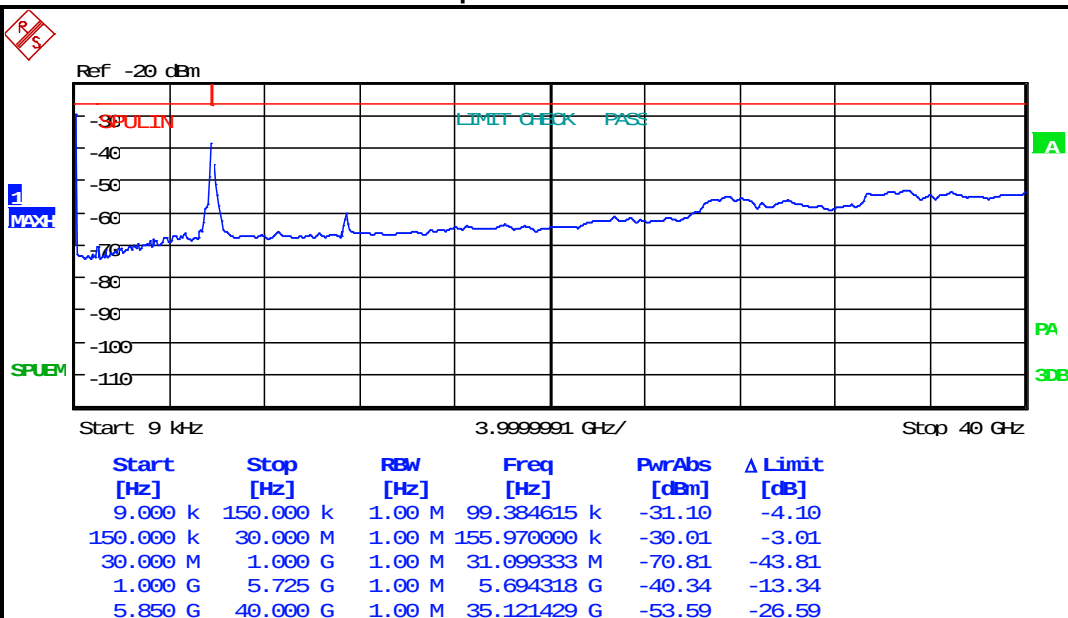
Plot 5-38: Antenna Conducted Spurious Emissions – 5745 MHz 802.11n 40 MHz BW
