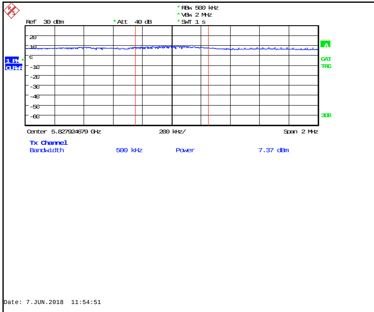
Plot 8-42: PSD – 5825 MHz 802.11a 20 MHz
