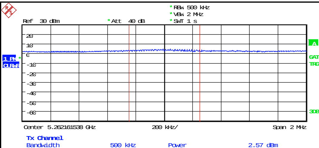
Plot 8-16: PSD – 5260 MHz 802.11n 40 MHz
