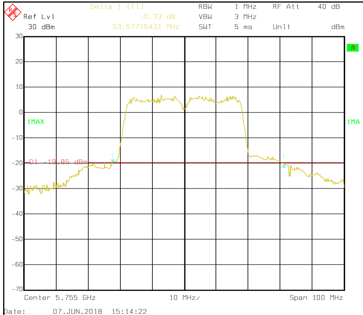
Plot 7-38: 99% OBW – 5755 MHz 802.11n 40 MHz BW
