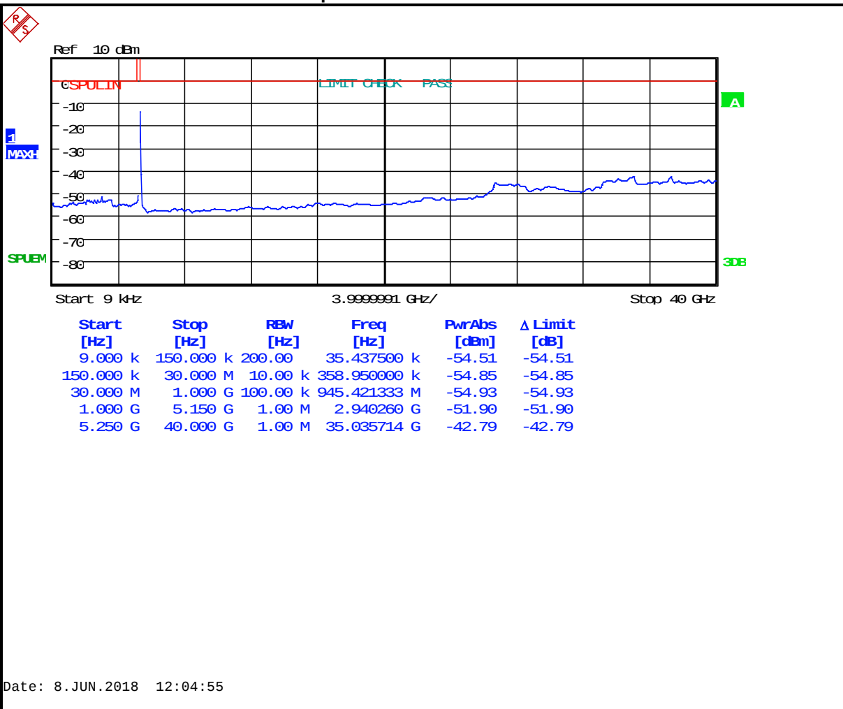
Plot 5-23: Antenna Conducted Spurious Emissions – 5290 MHz 802.11ac 80 MHz BW
