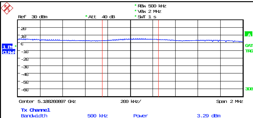
Plot 8-3: PSD – 5180 MHz 802.11n 40 MHz
