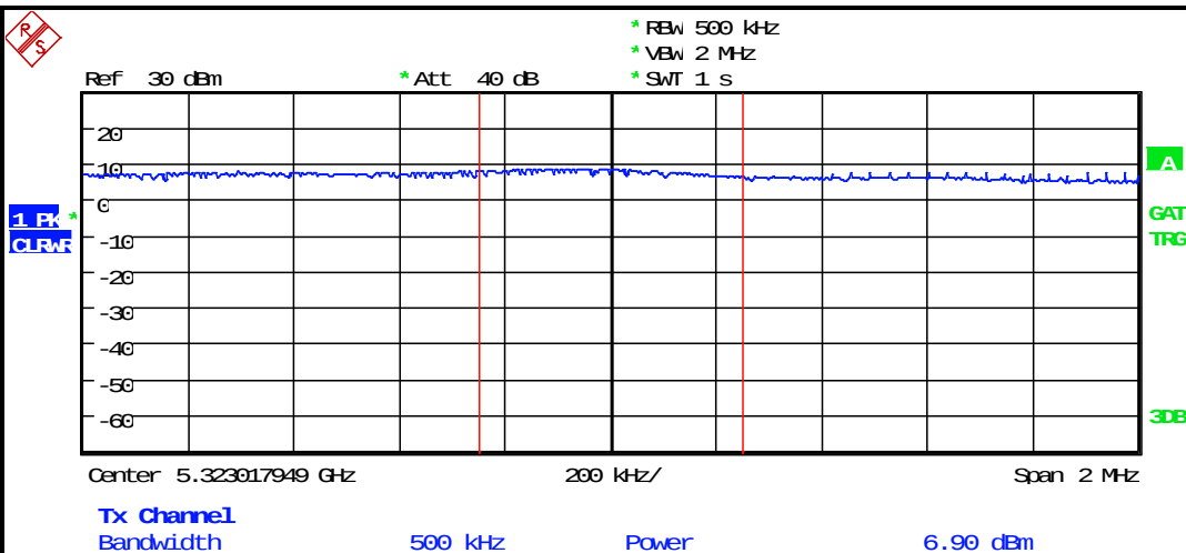
Plot 8-20: PSD – 5320 MHz 802.11a 20 MHz
