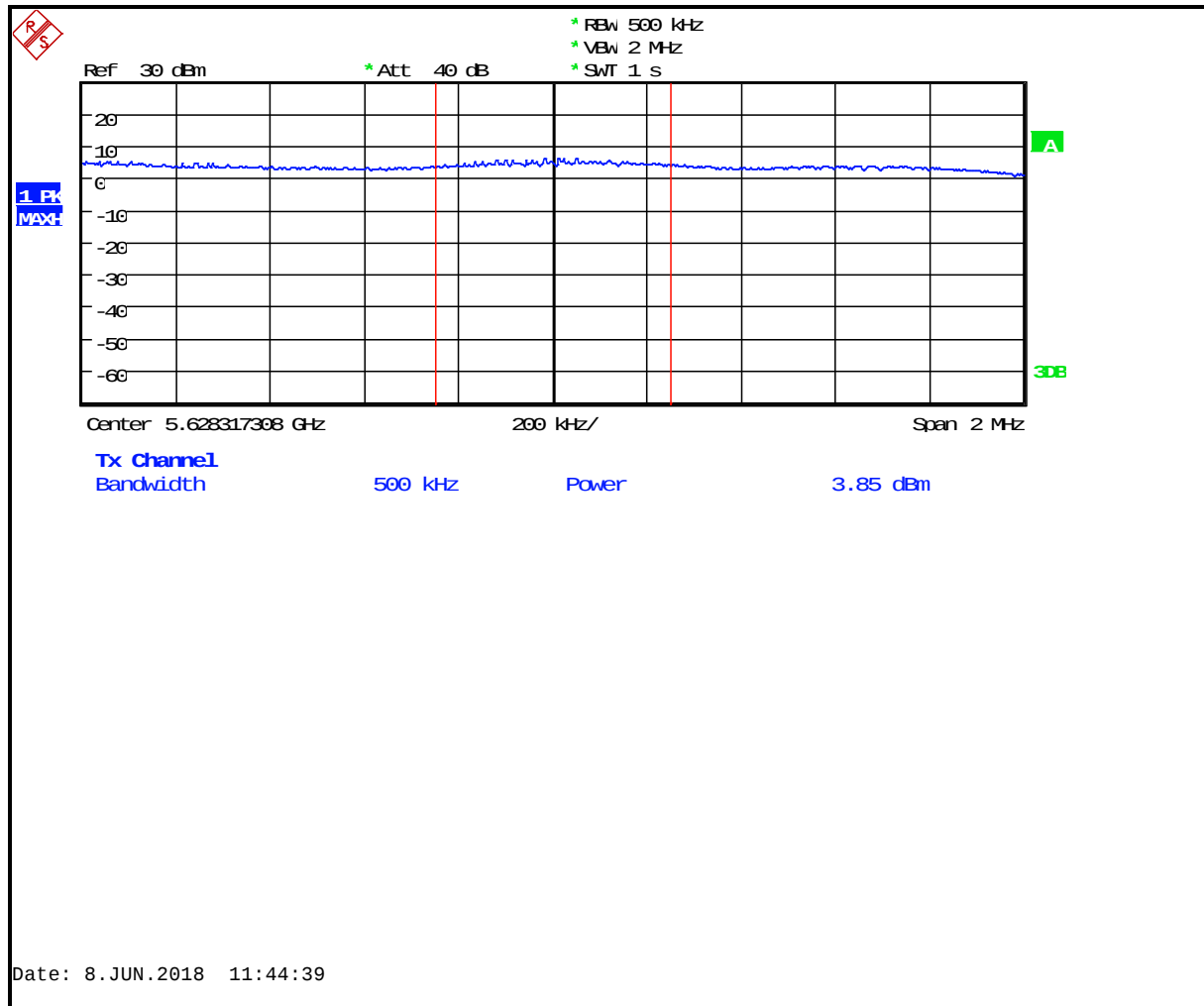
Plot 8-34: PSD – 5610 MHz 802.11ac 80 MHz
