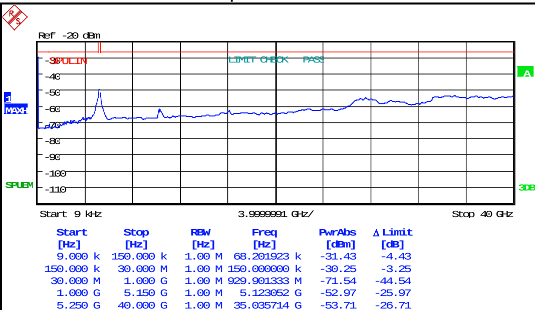
Plot 5-5: Antenna Conducted Spurious Emissions – 5200 MHz 802.11n 20 MHz BW
