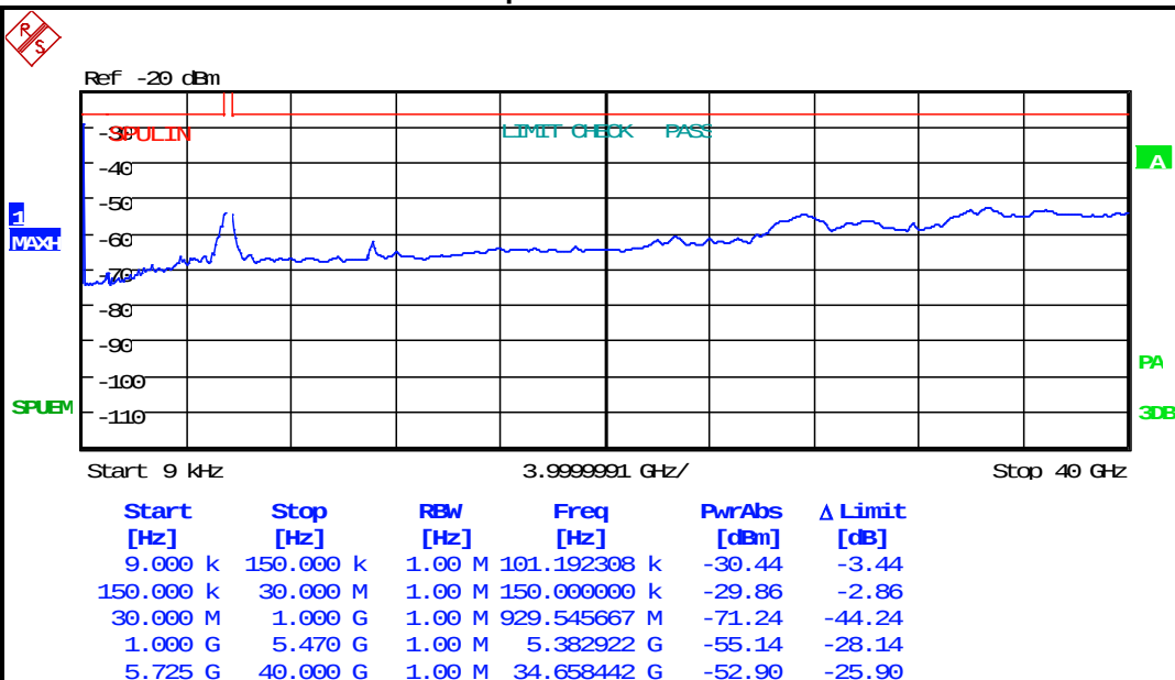
Plot 5-28: Antenna Conducted Spurious Emissions – 5600 MHz 802.11n 20 MHz BW
