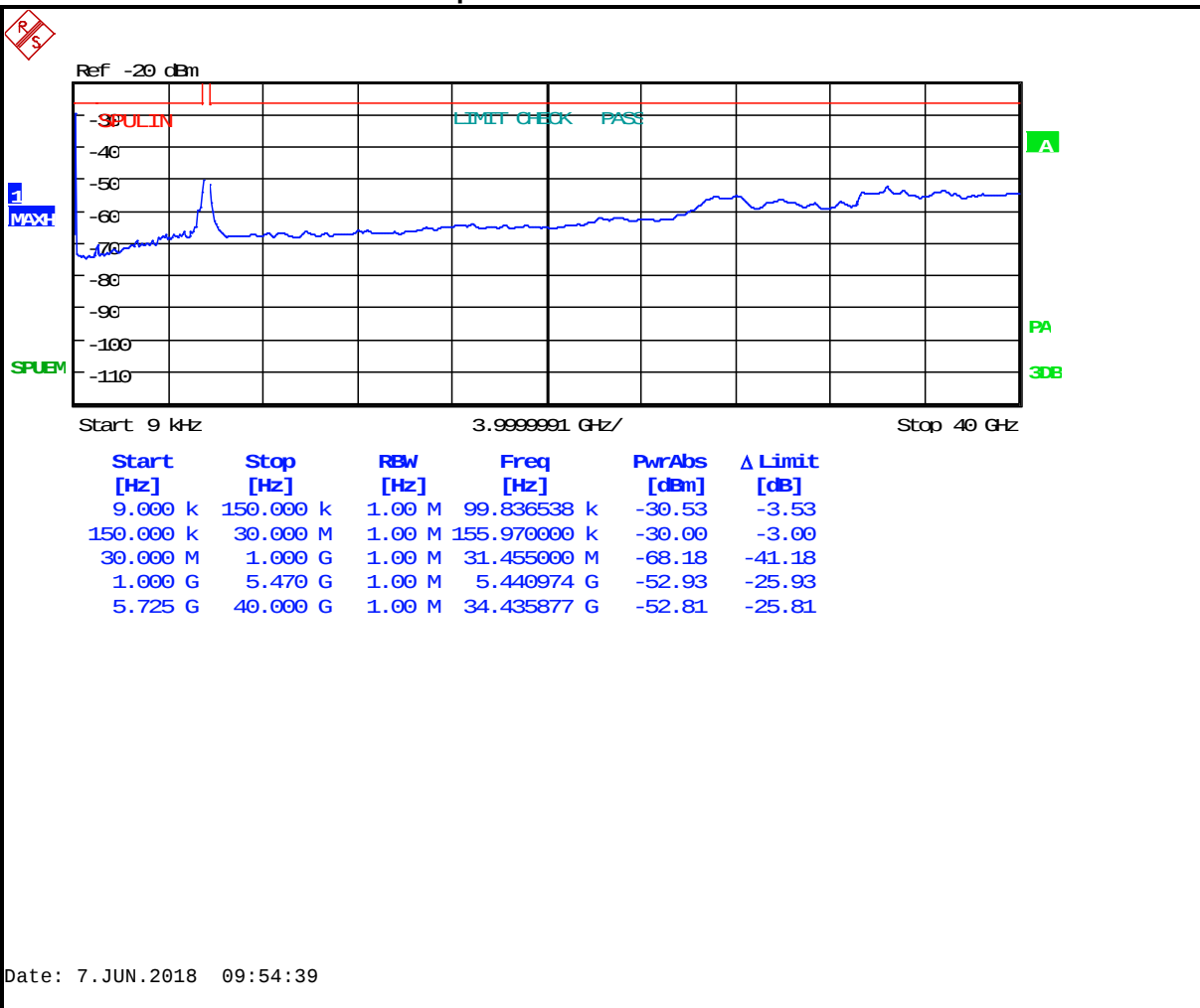
Plot 5-29: Antenna Conducted Spurious Emissions – 5600 MHz 802.11n 40 MHz BW
