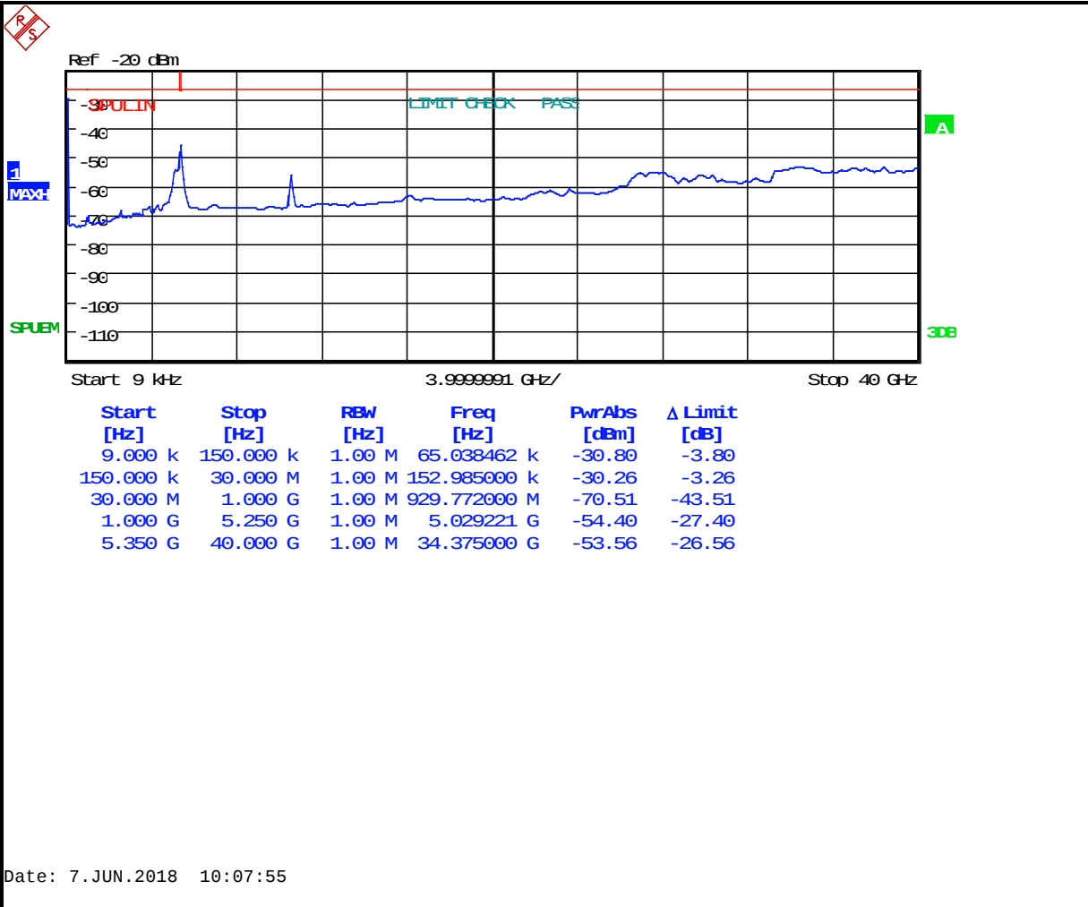
Plot 5-21: Antenna Conducted Spurious Emissions – 5320 MHz 802.11n 20 MHz BW
