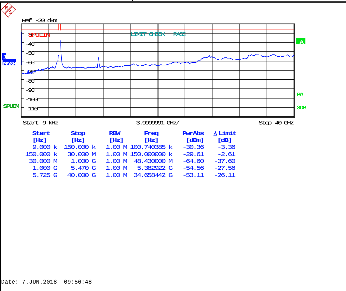
Plot 5-31: Antenna Conducted Spurious Emissions – 5700 MHz 802.11n 20 MHz BW
