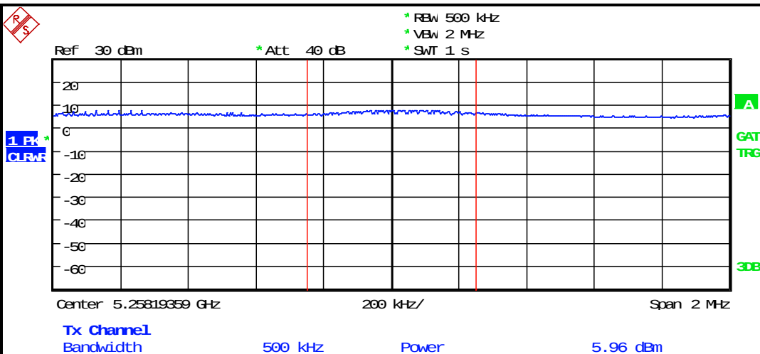
Plot 8-15: PSD – 5260 MHz 802.11n 20 MHz
