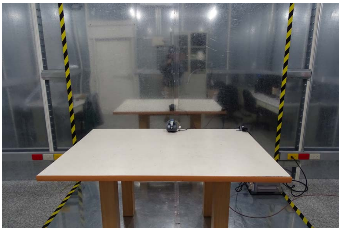
Back View of Conducted Test (Charger mode)
