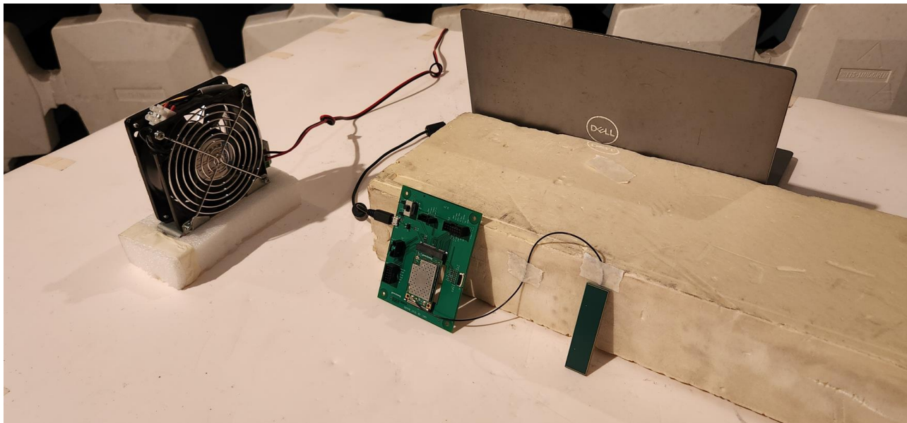
Radiated emission Test Setup – RFID Coupler (LUPUS32)
