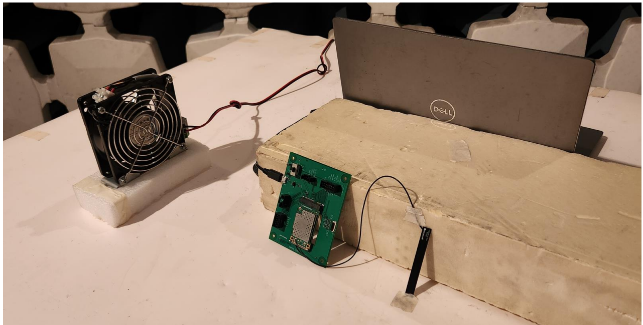
Radiated emission Test Setup – RFID Coupler (CORVUS10)
