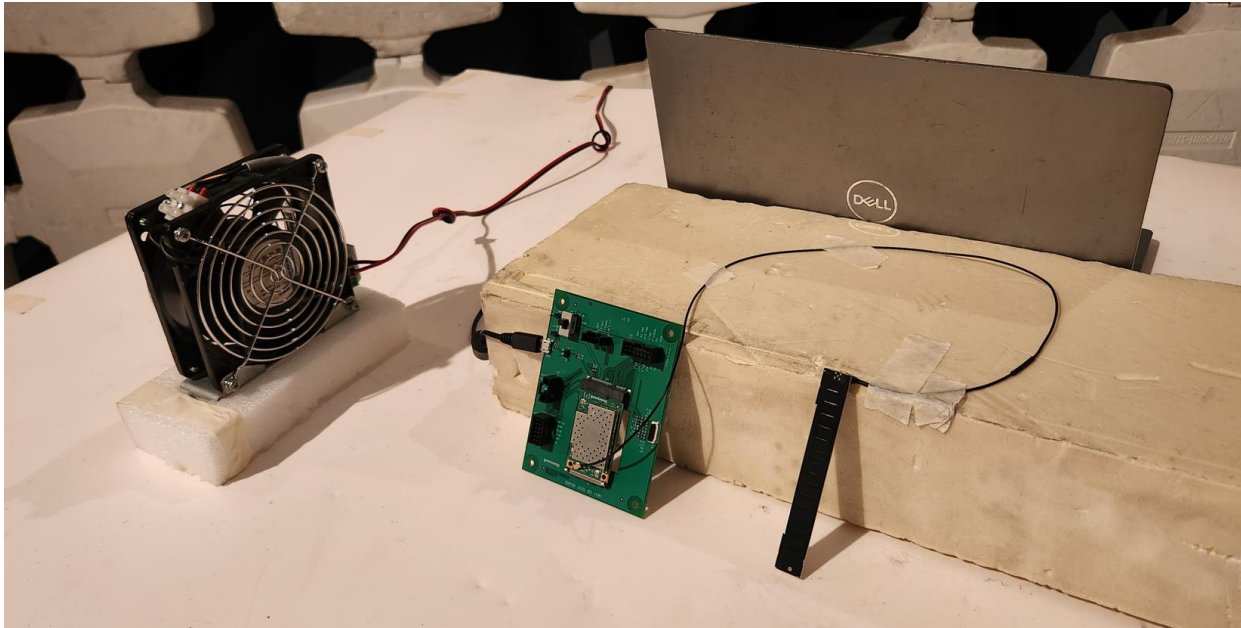
Radiated emission Test Setup – RFID Coupler (MAF95123-1 / 234-079-0600)
