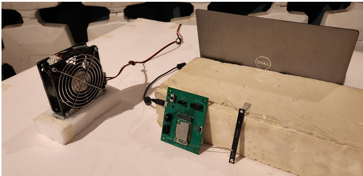
Radiated emission Test Setup – RFID Coupler (H2B1JH1A1H0200 / 710000068100)
