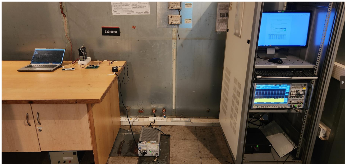
Conducted Emission Test setup on Power Lines (110VAC-60Hz)
