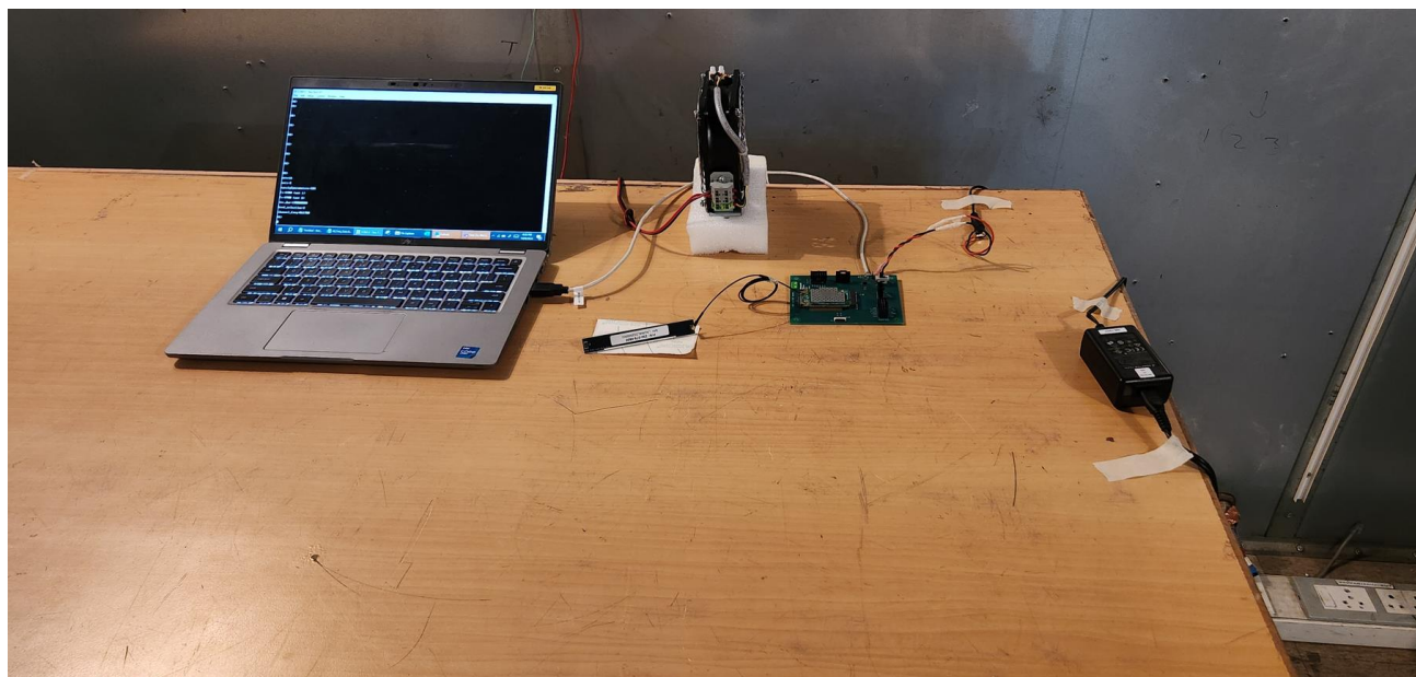
Conducted Emission Test setup on Power Lines - EUT arrangement on Test Table
