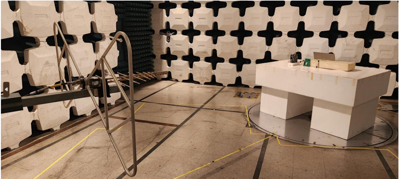
Radiated emission Test Setup – Horizontal Polarization
