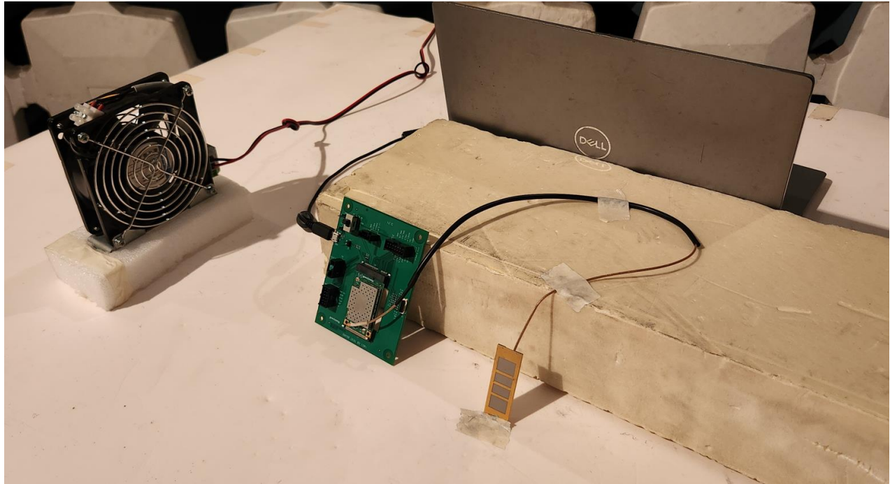
Radiated emission Test Setup – RFID Coupler (1-971140-001)
