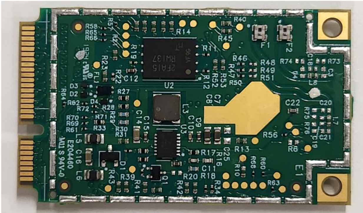
IM21-PRT RFID Module : Rear View without Shield
