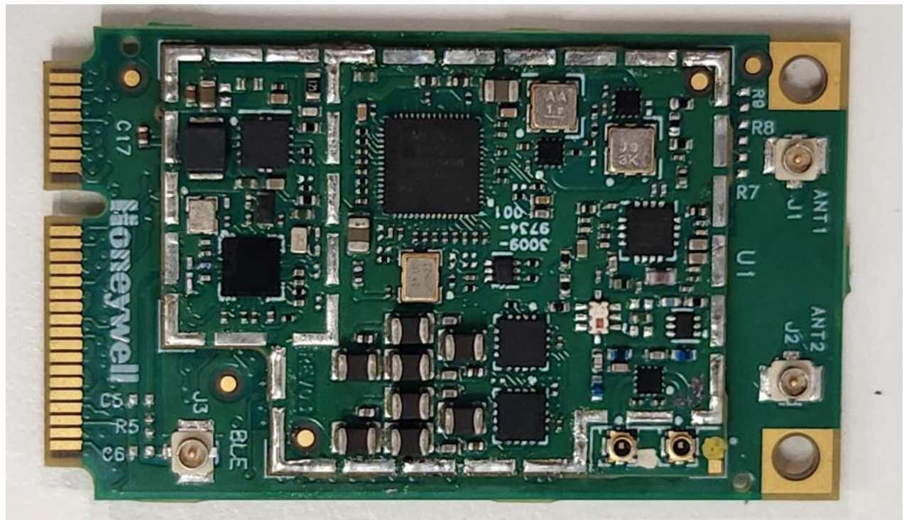
IM21-PRT RFID Module : Top View Without Shield
