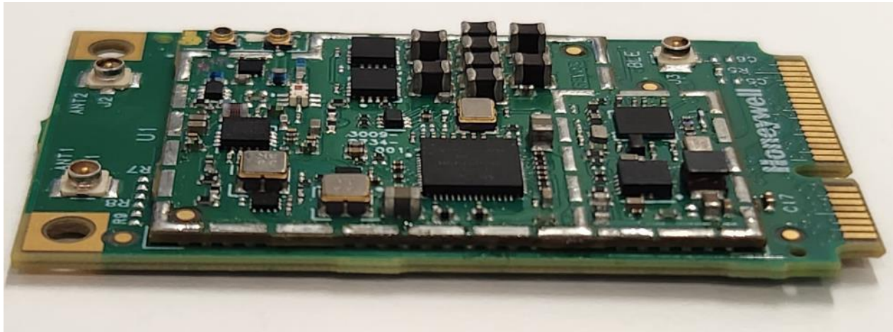
IM21-PRT RFID Module : Side View without shield
