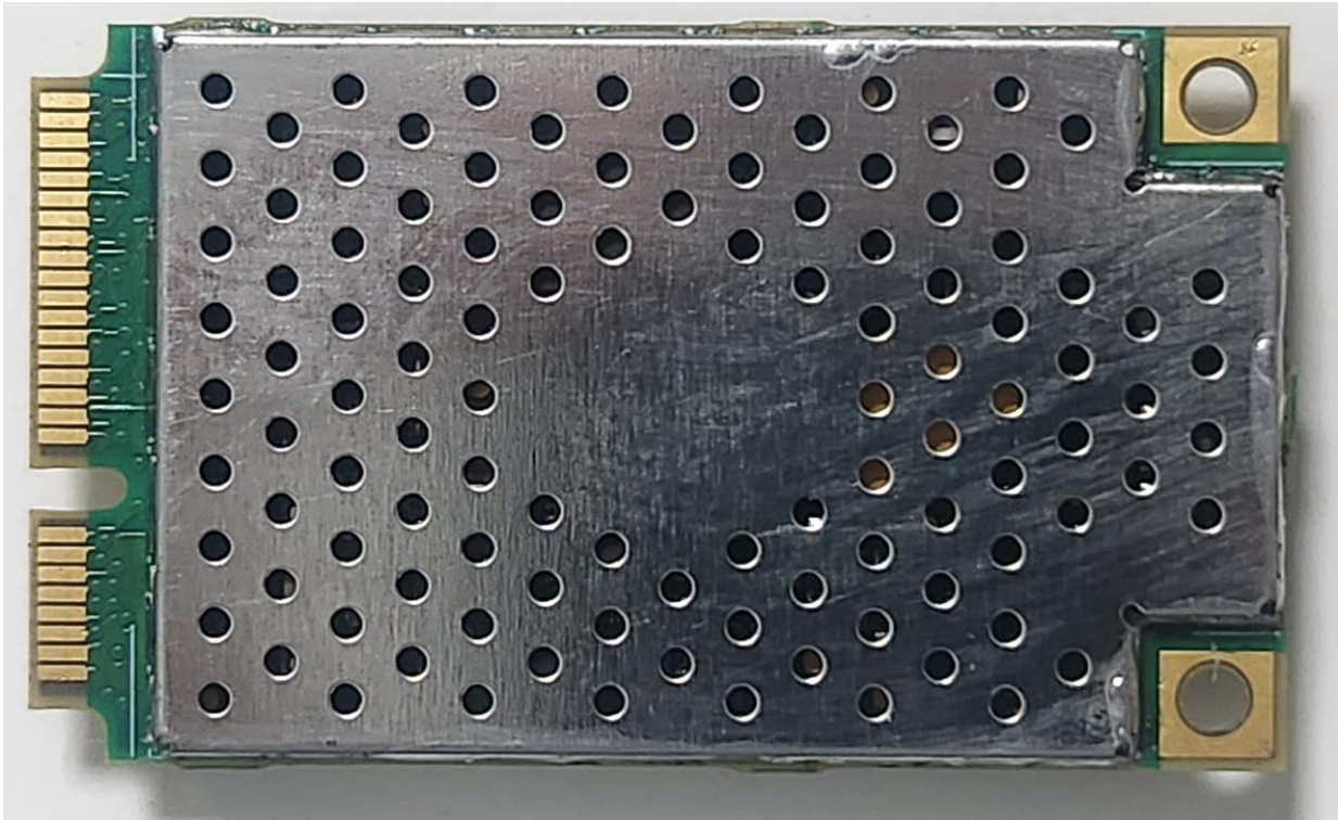
IM21-PRT RFID Module : Rear View
