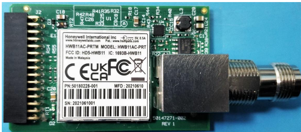
Top View of HWB11AC-PRT Module
