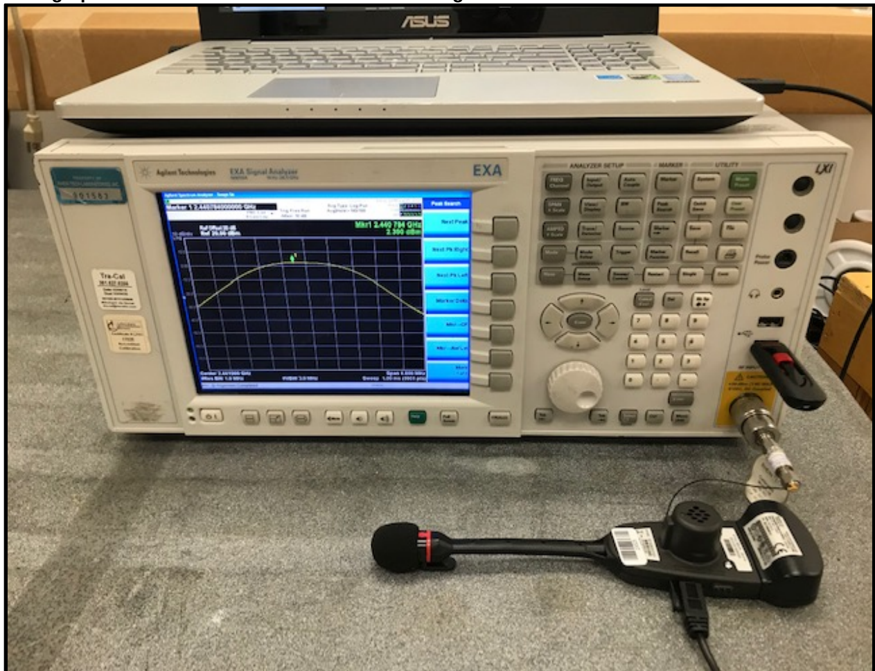
Photograph 3: Conducted Emissions Testing
