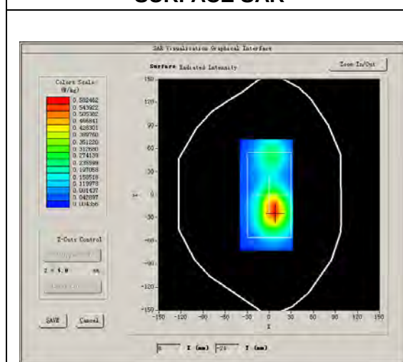
SURFACE SAR
