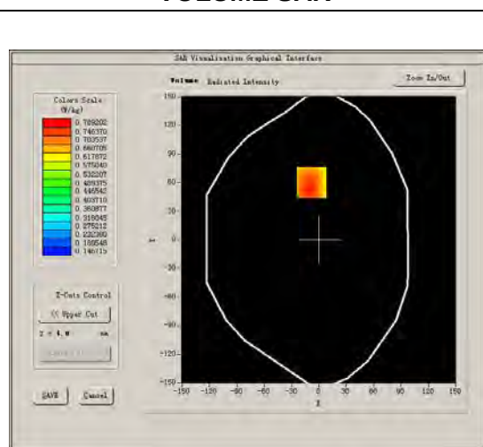
VOLUME SAR
