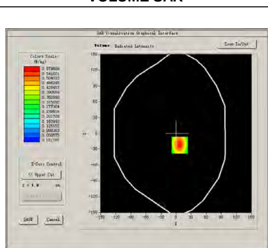
VOLUME SAR
