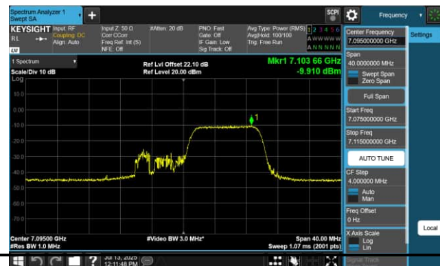
106 Tone_RU106_CH229 (7095MHz)
