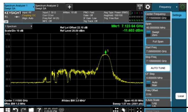
26 Tone_RU8_CH233 (7115MHz)
