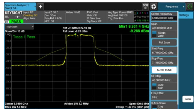
Channel 199 (6945MHz)
