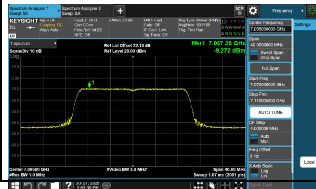
242 Tone_RU122_CH229 (7095MHz)
