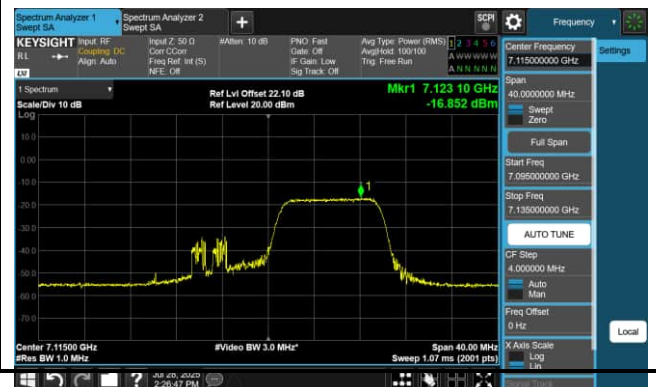
106 Tone_RU107_CH233 (7115MHz)
