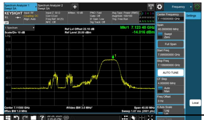
52 Tone_RU77_CH233 (7115MHz)
