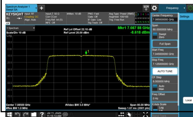
Channel 227 (7085MHz)
