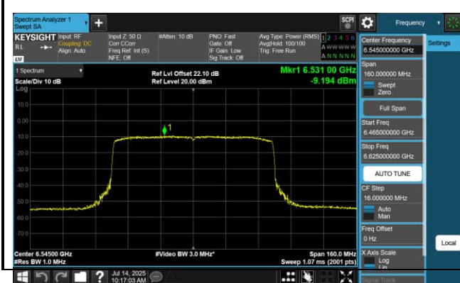
Channel 119 (6545MHz)
