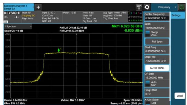
Channel 199 (6945MHz)
