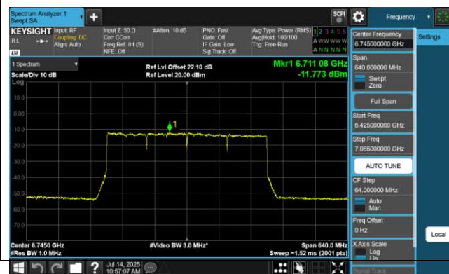
Channel 159 (6745MHz)
