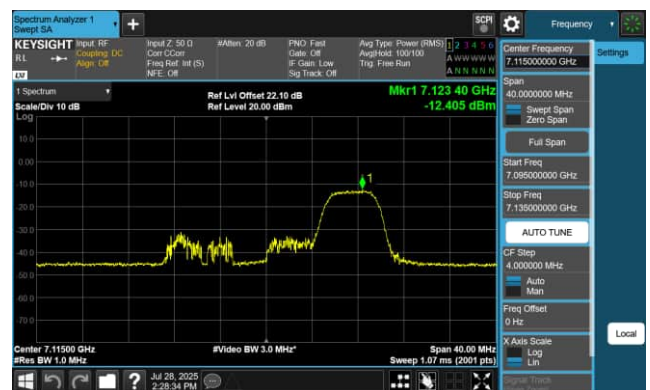
52 Tone_RU77_CH233 (7115MHz)
