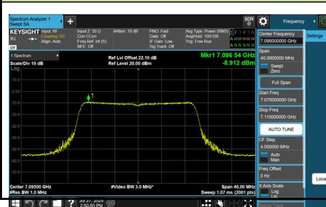
242 Tone_RU122_CH229 (7095MHz)
