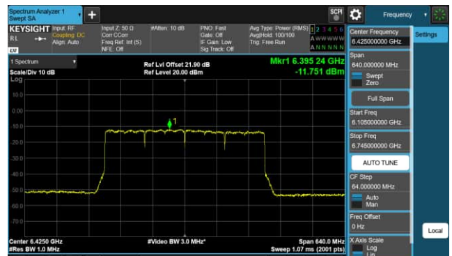
Channel 95 (6425MHz)
