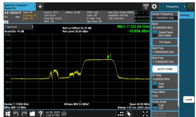
106 Tone_RU107_CH233 (7115MHz)
