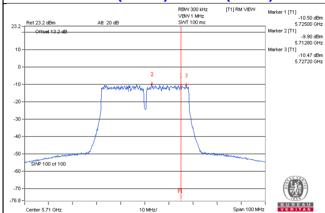
802.11ac (VHT40) / CH142 (UNII-3)
