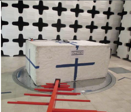
RADIATED FRONT PHOTO (BELOW 1 GHz)
