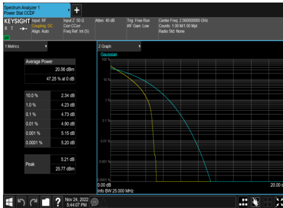
N7(20M)_DFT-s-OFDM_PI_2-BPSK_Outer_Full_High_CH
