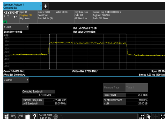
N77(90M)_CP-OFDM_256 QAM_Outer_Full_Mid_CH
