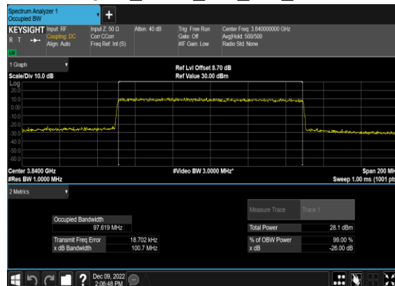
N77(100M)_CP-OFDM_16 QAM_Outer_Full_Mid_CH
