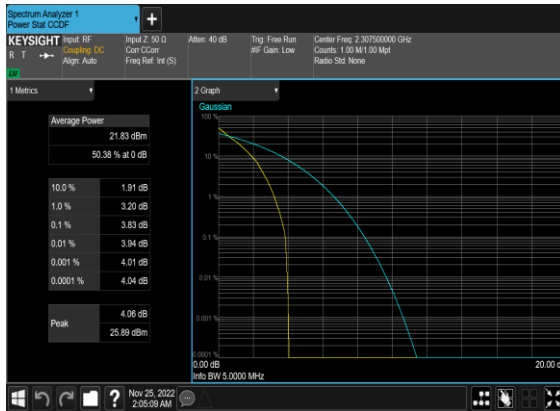
N30(5M)_DFT-s-OFDM_PI_2-BPSK_Outer_Full_Low_CH
