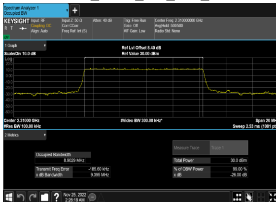
N30(10M)_DFT-s-OFDM_PI_2- BPSK_Outer_Full_Low_CH
