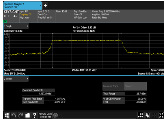
N30(5M)_DFT-s- OFDM_QPSK_Outer_Full_Mid_CH
