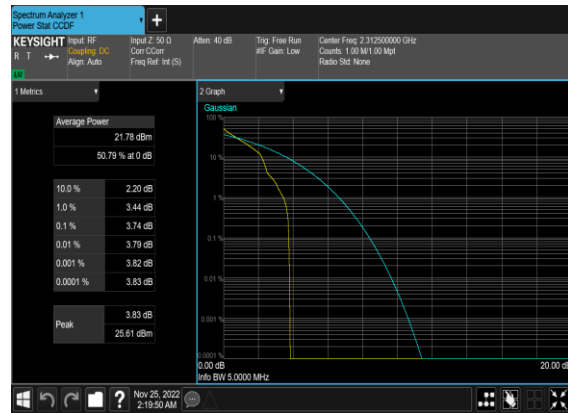
N30(5M)_DFT-s-OFDM_PI_2- BPSK_Edge_1RB_Left_High_CH
