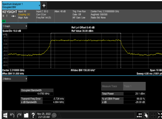
N30(5M)_DFT-s-OFDM_PI_2- BPSK_Outer_Full_Mid_CH
