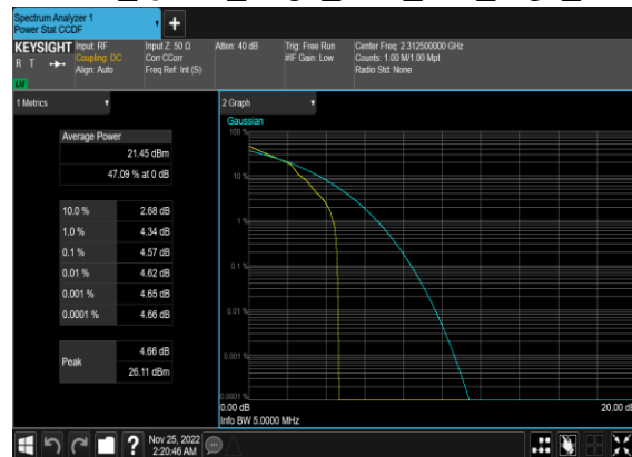
N30(5M)_DFT-s- OFDM_QPSK_Edge_1RB_Left_High_CH
