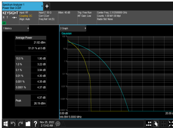
N30(5M)_DFT-s-OFDM_PI_2- BPSK_Outer_Full_High_CH
