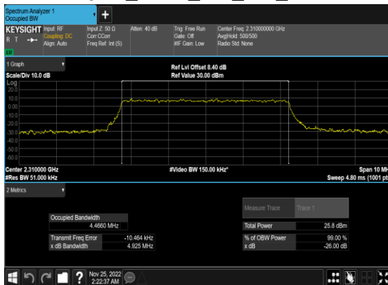
N30(5M)_CP-OFDM_64 QAM_Outer_Full_Mid_CH
