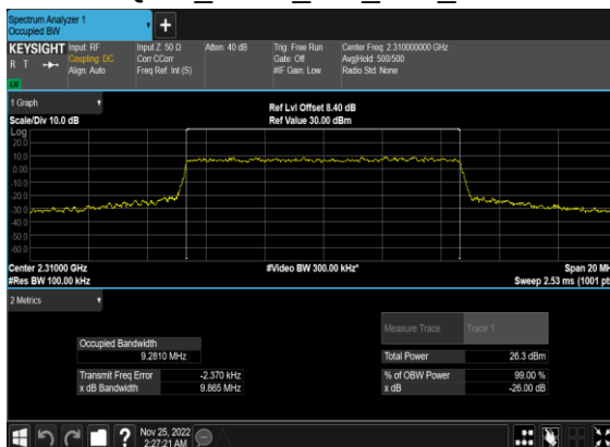
N30(10M)_CP-OFDM_64 QAM_Outer_Full_Low_CH
