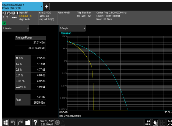
N30(5M)_DFT-s- OFDM_QPSK_Outer_Full_High_CH
