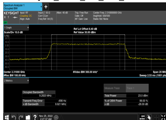
N30(10M)_CP-OFDM_256 QAM_Outer_Full_Low_CH
