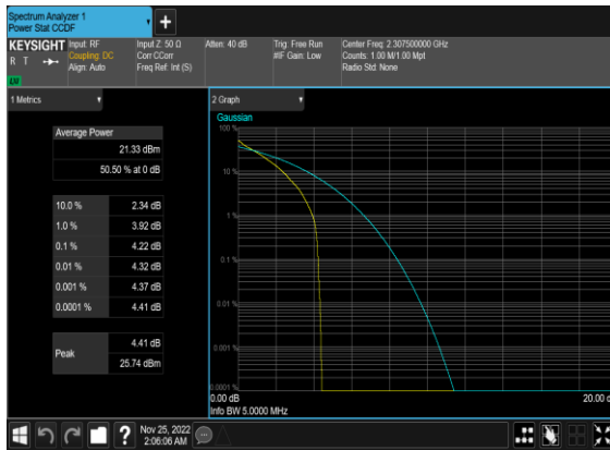
N30(5M)_DFT-s-OFDM_QPSK_Outer_Full_Low_CH
