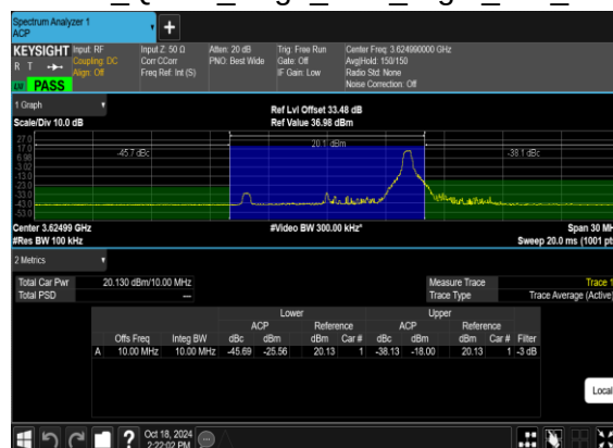
N48(10M)_DFT-s- OFDM_QPSK_Edge_1RB_Right_Mid_CH
