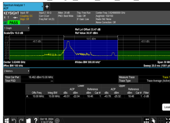
N48(10M)_DFT-s-OFDM_PI_2- BPSK_Edge_1RB_Left_Mid_CH
