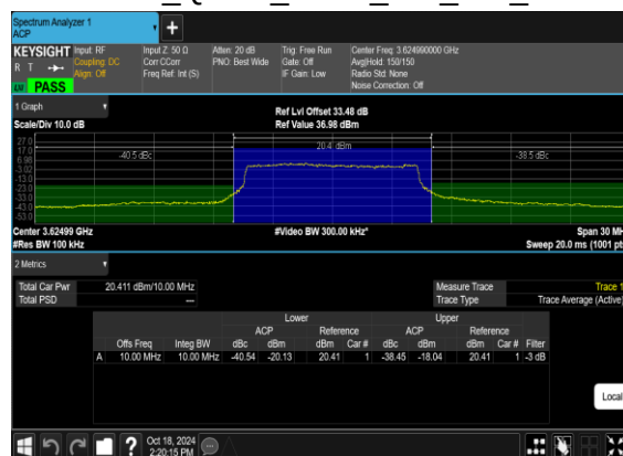
N48(10M)_DFT-s- OFDM_QPSK_Outer_Full_Mid_CH
