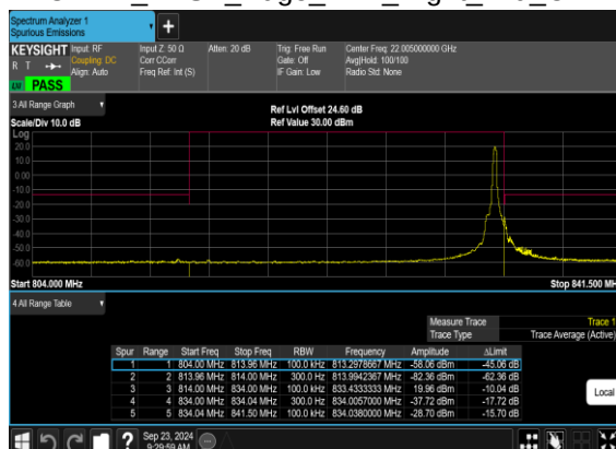
N26(20M)_DFT-s- OFDM_BPSK_Edge_1RB_Right_Mid_CH
