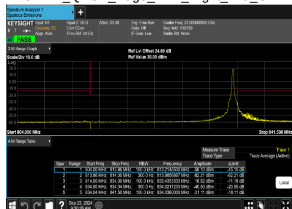
N26(20M)_DFT-s- OFDM_QPSK_Edge_1RB_Right_Mid_CH
