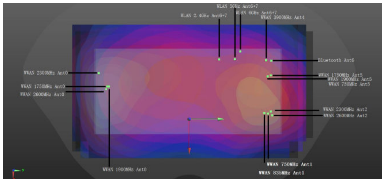
Body worn WWAN+FR1+BT+WLAN2.4GHz+ WLAN5 GHz/6 GHz 10mm
