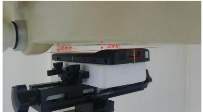
Back, Test Separation 16 mm
