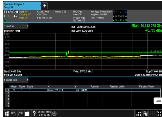
N48(30M)_DFT-s- OFDM_BPSK_Edge_1RB_Left_Low_CH
