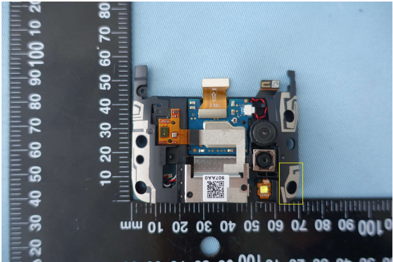
Ant 6 BT/Wlan
