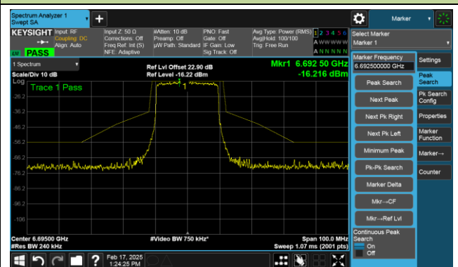
Channel 149 (6695MHz)
