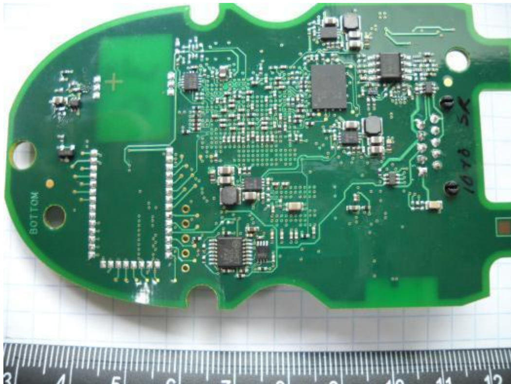
Fig.4: PCB View-1
