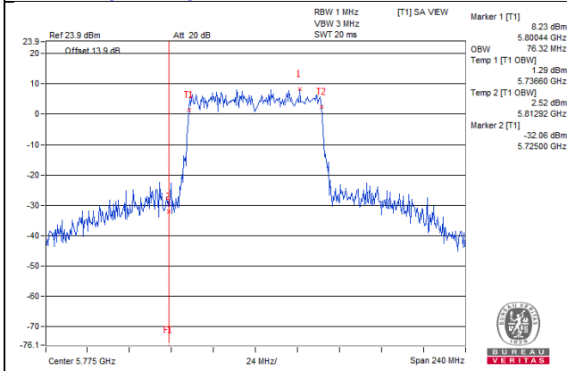
802.11ac(VHT80)_Chain0 / CH155
