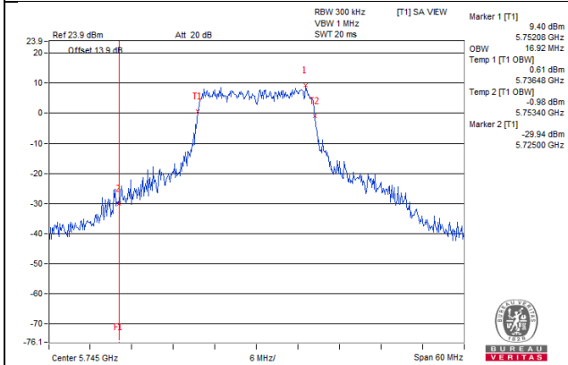
802.11ac(VHT20)_Chain0 / CH149
