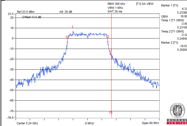
802.11ac(VHT20)_Chain0 / CH48
