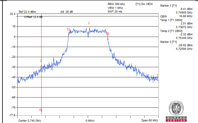
802.11ac(VHT20)_Chain1 / CH149
