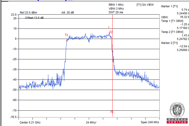
802.11ac(VHT80)_Chain0 / CH42
