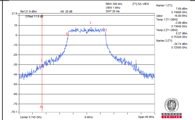
802.11ac(VHT20)_Chain1 / CH149
