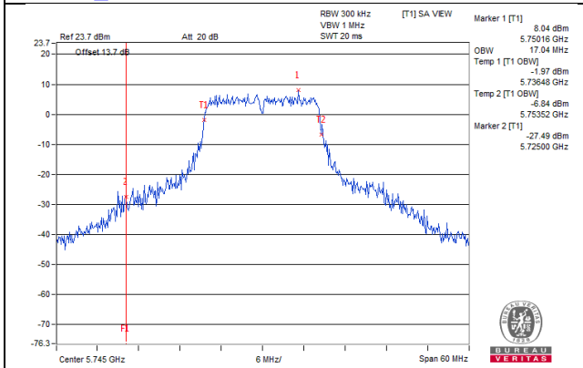
802.11ac(VHT20)_Chain0 / CH149
