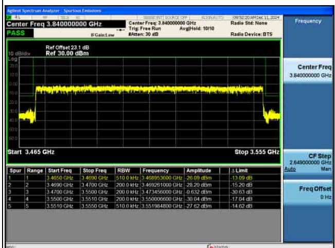
EDGE_MIMO(ANT5)_n77(K)_30KHz_QPSK_80M_FULL RB@0_CH634000
