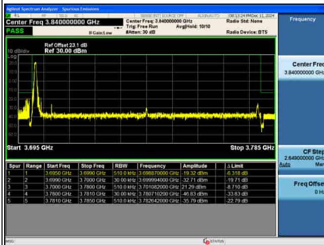
EDGE_MIMO(ANT5)_n77(N)_30KHz_QPSK_80M_1RB@MAX_CH649334
