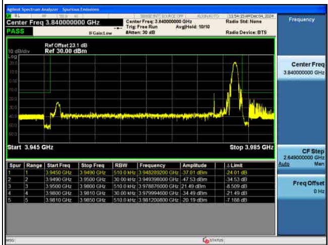
EDGE_5G_n77(N)_30KHz_P12-BPSK_30M_FULL RB@0_CH664332
