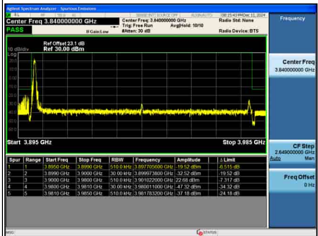
EDGE_MIMO(ANT5)_n77(N)_30KHz_QPSK_80M_1RB@MAX_CH662666
