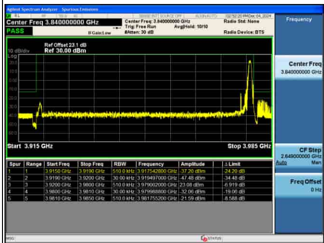
EDGE_5G_n77(N)_30KHz_P12-BPSK_60M_FULL RB@0_CH663332
