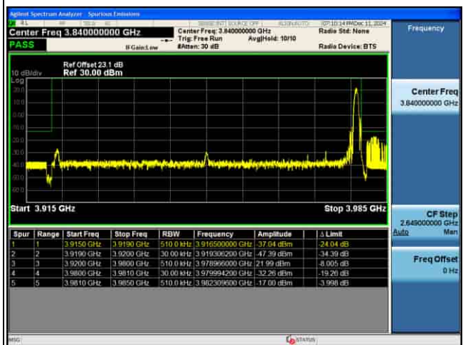
EDGE_MIMO(ANT5)_n77(N)_30KHz_QPSK_60M_FULL RB@0_CH663332
