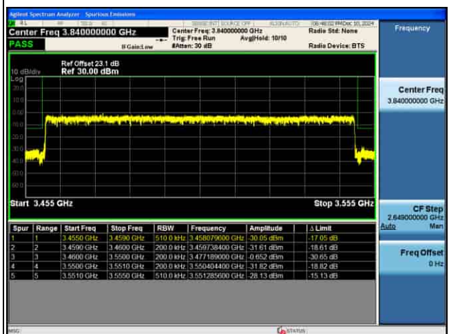
EDGE_MIMO(ANT5)_n77(K)_30KHz_QPSK_90M_FULL RB@0_CH633666
