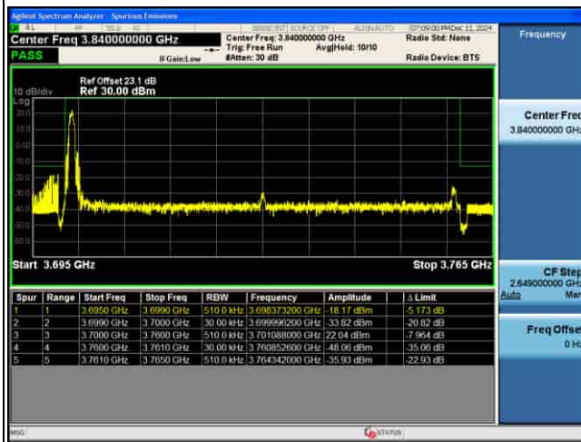
EDGE_MIMO(ANT5)_n77(N)_30KHz_QPSK_60M_1RB@MAX_CH648668
