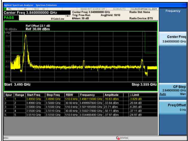
EDGE_MIMO(ANT5)_n77(K)_30KHz_QPSK_50M_1RB@MAX_CH635000
