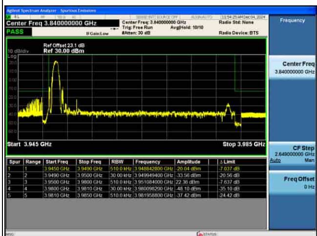
EDGE_5G_n77(N)_30KHz_P12-BPSK_30M_1RB@0_CH664332
