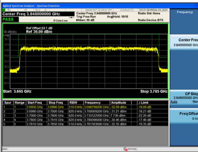
EDGE_5G_n77(N)_30KHz_P12-BPSK_90M_1RB@0_CH649668
