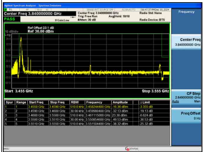
EDGE_MIMO(ANT5)_n77(K)_30KHz_QPSK_90M_1RB@MAX_CH633666
