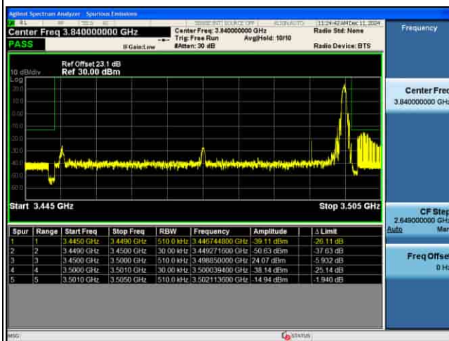
EDGE_MIMO(ANT5)_n77(K)_30KHz_QPSK_50M_FULL RB@0_CH631668
