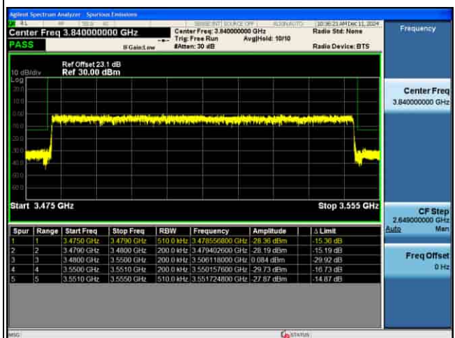
EDGE_MIMO(ANT5)_n77(K)_30KHz_QPSK_70M_FULL RB@0_CH634332
