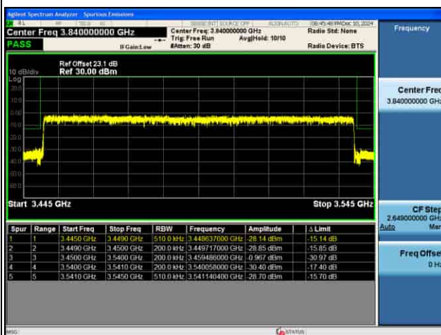
EDGE_MIMO(ANT5)_n77(K)_30KHz_QPSK_90M_FULL RB@0_CH633000
