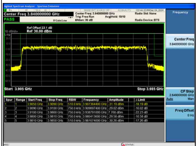
EDGE_5G_n77(N)_30KHz_P12-BPSK_70M_FULL RB@MAX_CH663000
