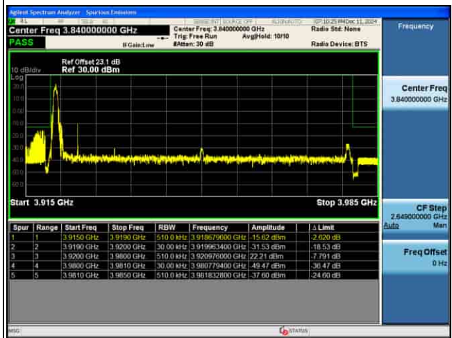
EDGE_MIMO(ANT5)_n77(N)_30KHz_QPSK_60M_1RB@MAX_CH663332
