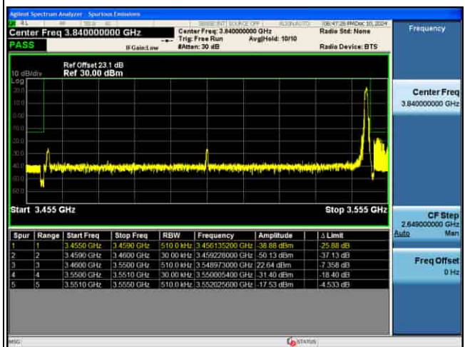
EDGE_MIMO(ANT5)_n77(K)_30KHz_QPSK_90M_FULL RB@0_CH633666
