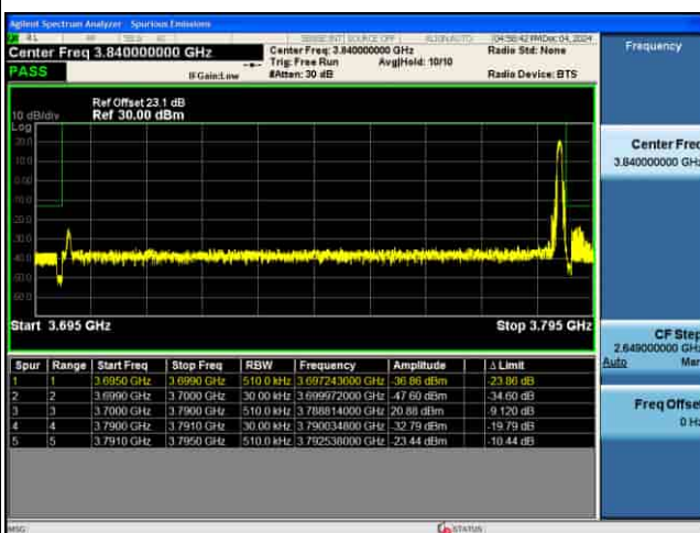
EDGE_5G_n77(N)_30KHz_P12-BPSK_90M_1RB@MAX_CH649668
