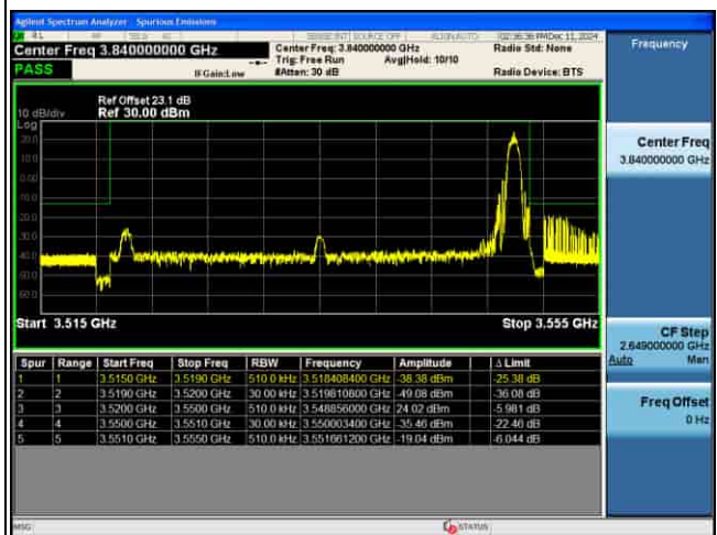
EDGE_MIMO(ANT5)_n77(K)_30KHz_QPSK_30M_FULL RB@0_CH635666
