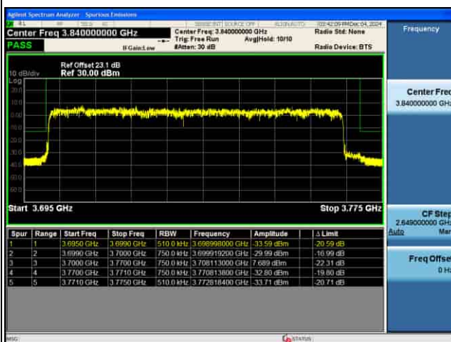
EDGE_5G_n77(N)_30KHz_P12-BPSK_70M_FULL RB@MAX_CH649000
