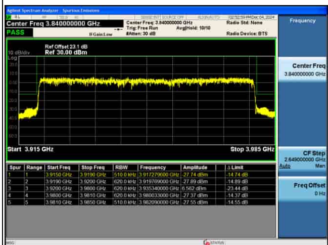
EDGE_5G_n77(N)_30KHz_P12-BPSK_70M_1RB@0_CH663000
