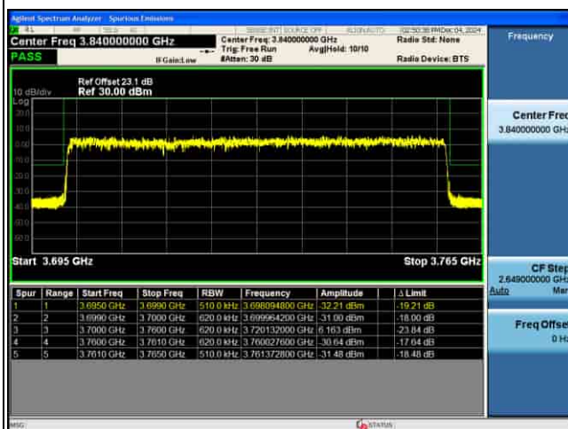
EDGE_5G_n77(N)_30KHz_P12-BPSK_70M_1RB@0_CH649000
