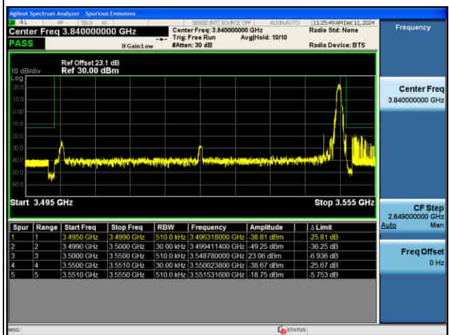
EDGE_MIMO(ANT5)_n77(K)_30KHz_QPSK_50M_FULL RB@0_CH635000
