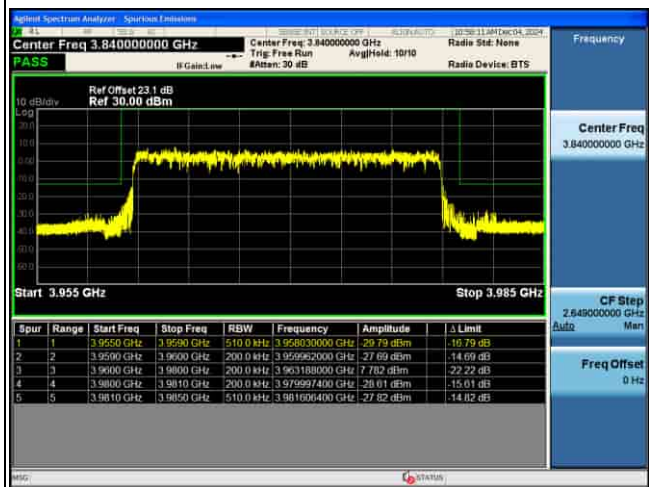
EDGE_5G_n77(N)_30KHz_P12-BPSK_20M_FULL RB@MAX_CH664666
