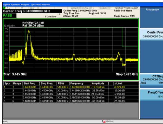
EDGE_MIMO(ANT5)_n77(K)_30KHz_QPSK_30M_1RB@MAX_CH631000
