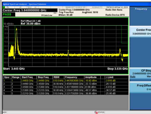
EDGE_MIMO(ANT5)_n77(K)_30KHz_QPSK_80M_1RB@MAX_CH632668
