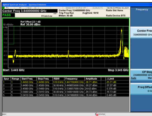
EDGE_MIMO(ANT5)_n77(K)_30KHz_QPSK_90M_FULL RB@0_CH633000
