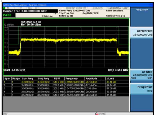
EDGE_MIMO(ANT5)_n77(K)_30KHz_QPSK_50M_FULL RB@0_CH635000
