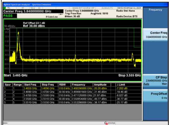
EDGE_MIMO(ANT5)_n77(K)_30KHz_QPSK_80M_1RB@MAX_CH634000
