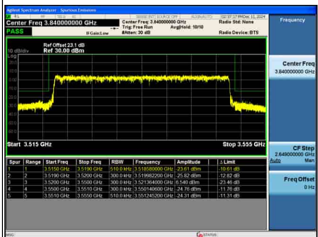
EDGE_MIMO(ANT5)_n77(K)_30KHz_QPSK_30M_FULL RB@0_CH635666
