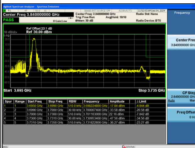
EDGE_5G_n77(N)_30KHz_P12-BPSK_30M_1RB@0_CH647668
