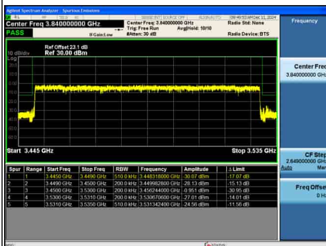
EDGE_MIMO(ANT5)_n77(K)_30KHz_QPSK_80M_FULL RB@0_CH632668
