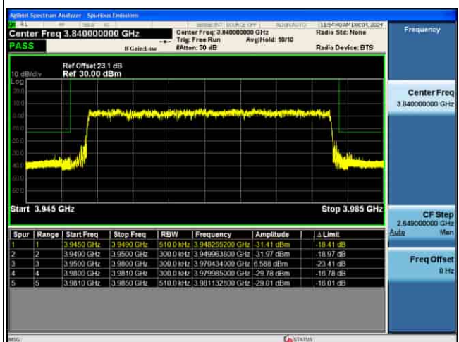
EDGE_5G_n77(N)_30KHz_P12-BPSK_30M_FULL RB@MAX_CH664332
