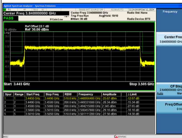
EDGE_MIMO(ANT5)_n77(K)_30KHz_QPSK_50M_FULL RB@0_CH631668
