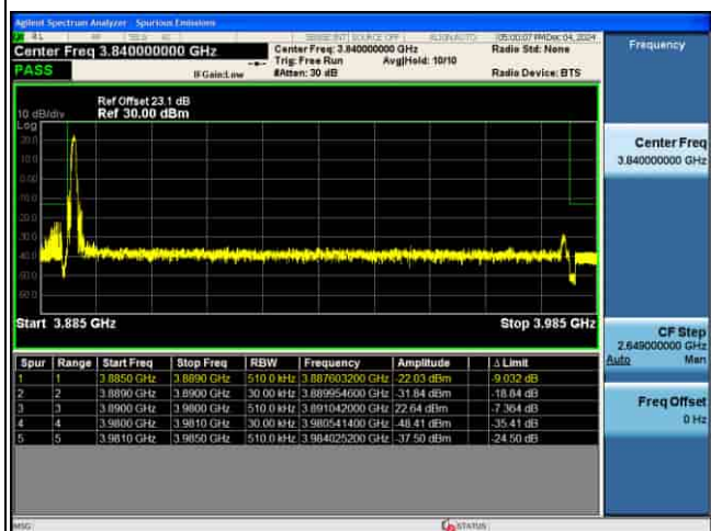
EDGE_5G_n77(N)_30KHz_P12-BPSK_90M_1RB@MAX_CH662332
