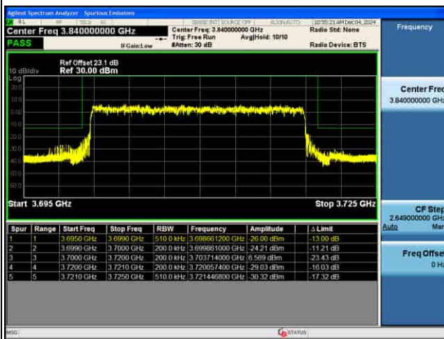
EDGE_5G_n77(N)_30KHz_P12-BPSK_20M_FULL RB@MAX_CH647334
