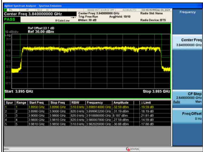
EDGE_5G_n77(N)_30KHz_P12-BPSK_90M_1RB@0_CH662332
