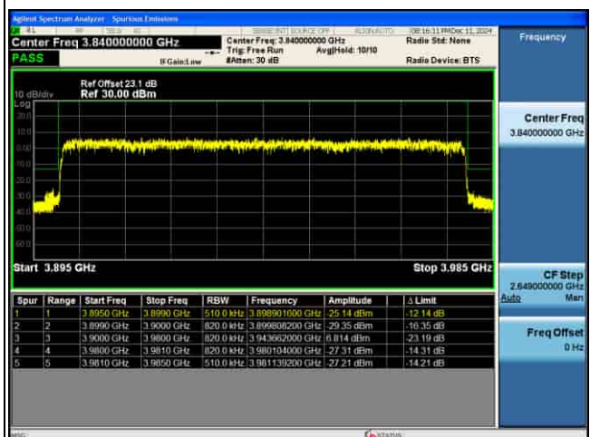
EDGE_MIMO(ANT5)_n77(N)_30KHz_QPSK_80M_FULL RB@0_CH662666
