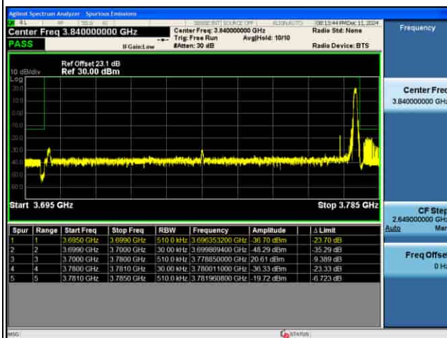
EDGE_MIMO(ANT5)_n77(N)_30KHz_QPSK_80M_FULL RB@0_CH649334
