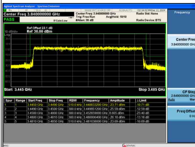
EDGE_MIMO(ANT5)_n77(K)_30KHz_QPSK_30M_FULL RB@0_CH631000
