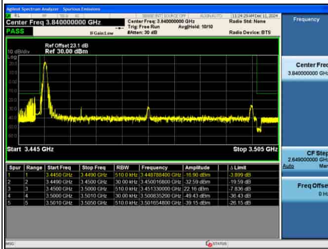
EDGE_MIMO(ANT5)_n77(K)_30KHz_QPSK_50M_1RB@MAX_CH631668
