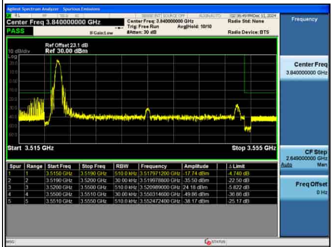
EDGE_MIMO(ANT5)_n77(K)_30KHz_QPSK_30M_1RB@MAX_CH635666
