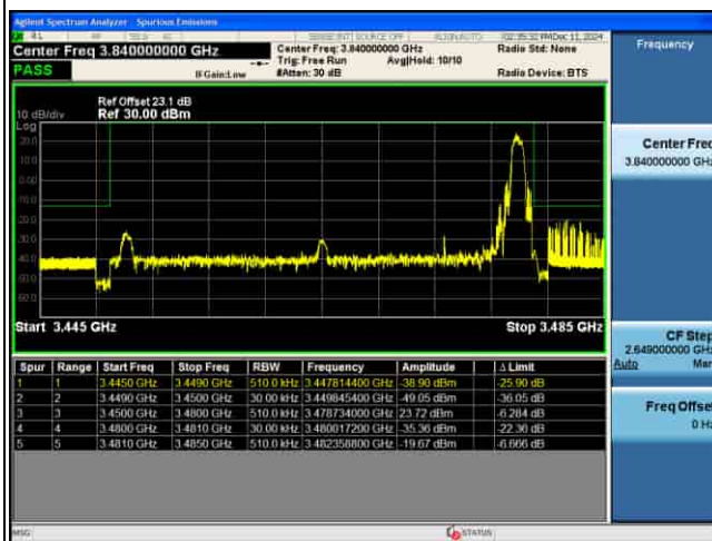
EDGE_MIMO(ANT5)_n77(K)_30KHz_QPSK_30M_FULL RB@0_CH631000
