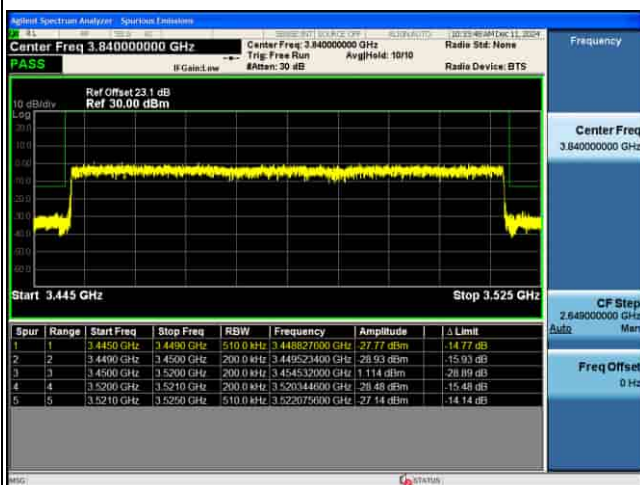
EDGE_MIMO(ANT5)_n77(K)_30KHz_QPSK_70M_FULL RB@0_CH632334
