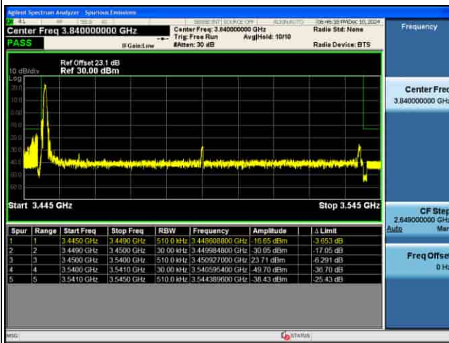
EDGE_MIMO(ANT5)_n77(K)_30KHz_QPSK_90M_1RB@MAX_CH633000
