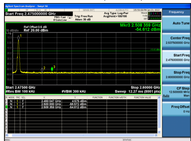
Mode 1 CH39(2480MHz)
