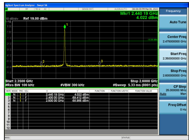
Mode 1 CH19(2440MHz)
