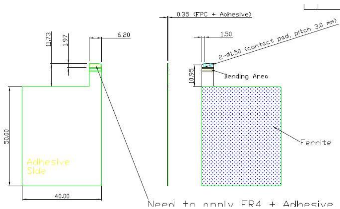
NFC Antenna (Extended Battery Door on Left, Standard Battery Door on Right)
