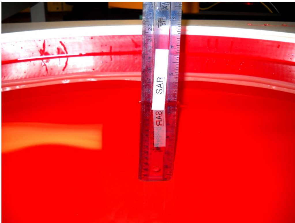
Photo 10: 15cm Liquid Depth in Elliptical Phantom
