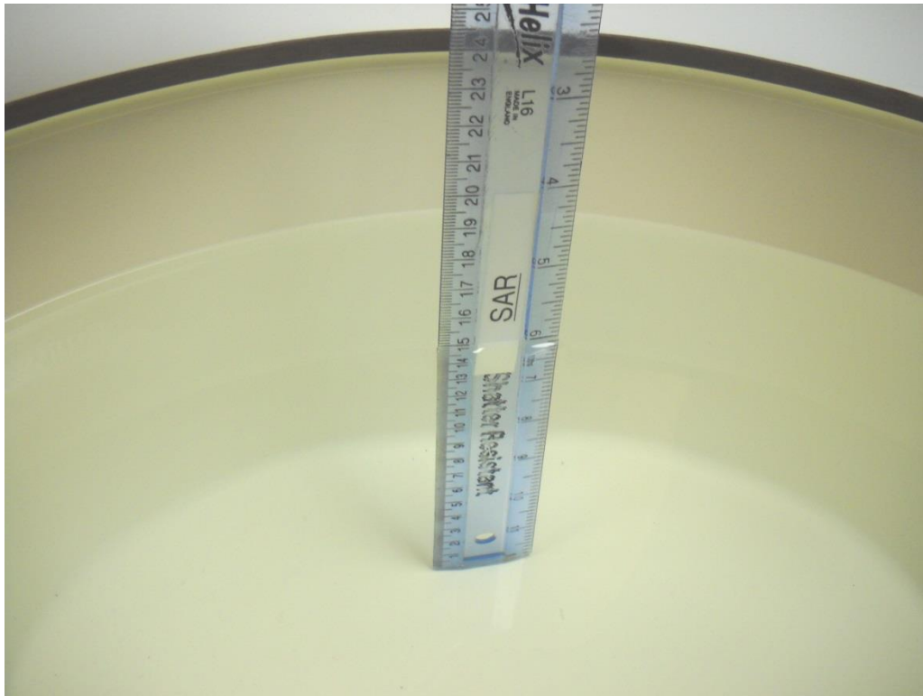
Photo 9: 15cm Liquid Depth in Flat Section of SAM Phantom
