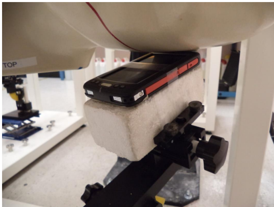
Photo 2: Left Tilt 15° under SAM Phantom Left Head
