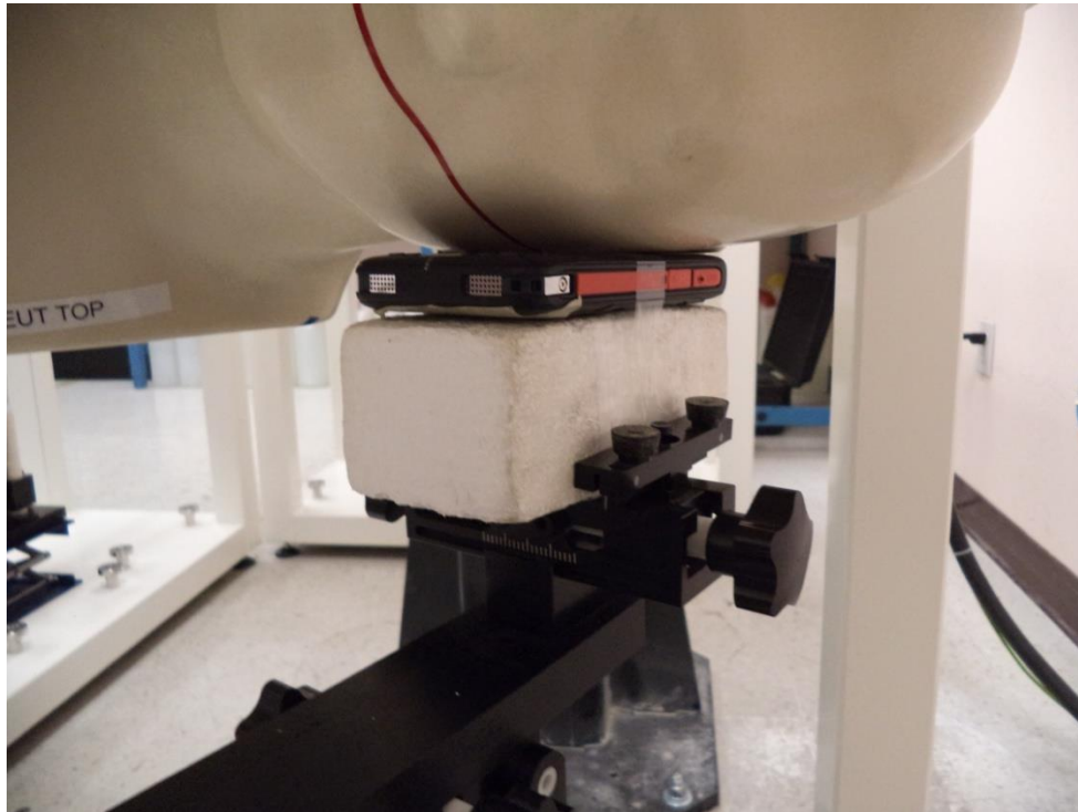
Photo 1: Left Touch under SAM Phantom Left Head
