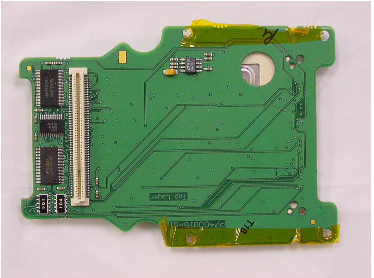
Rear View of WLAN Daughter Board
