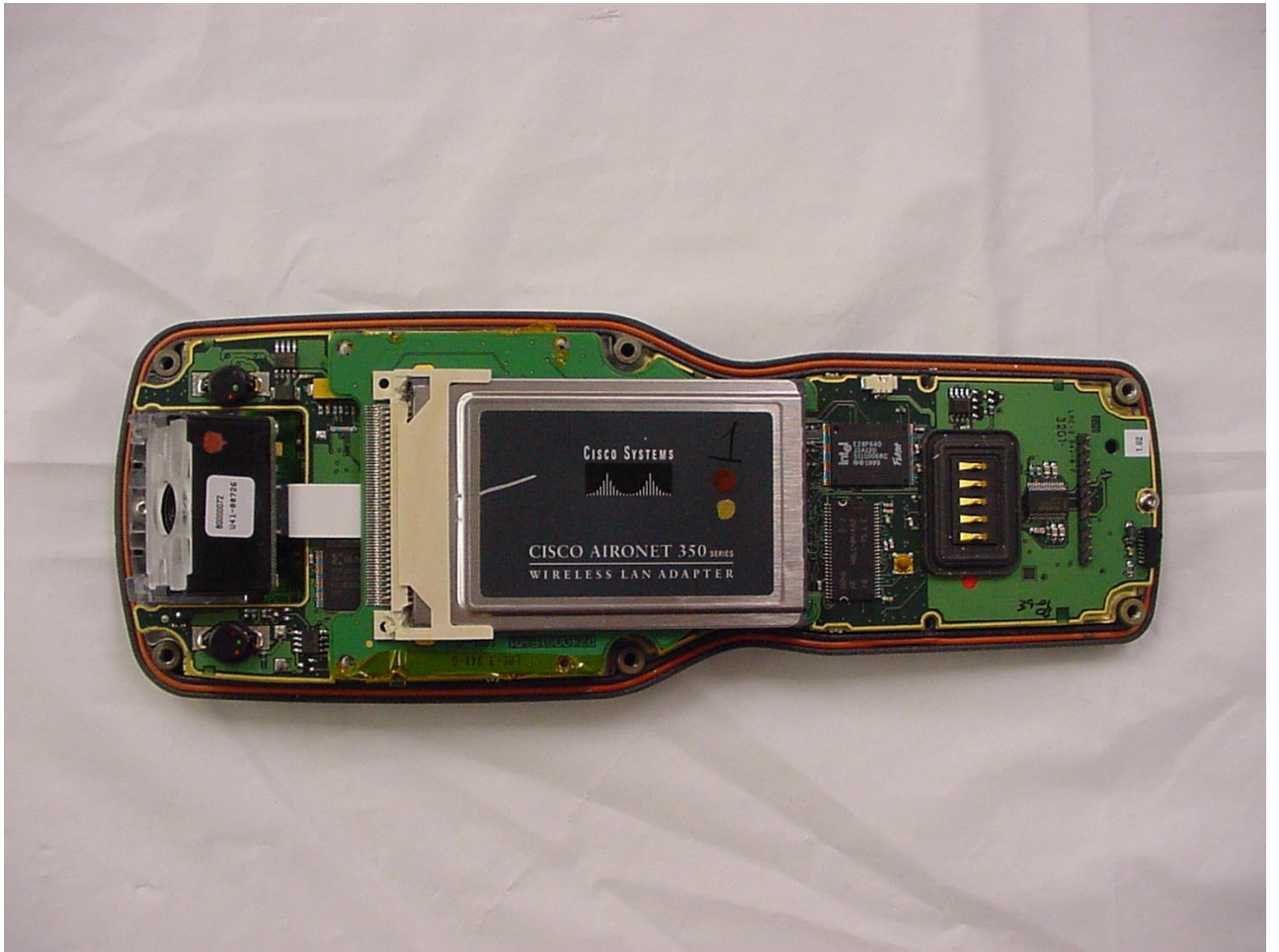
Inside View with WLAN Card
