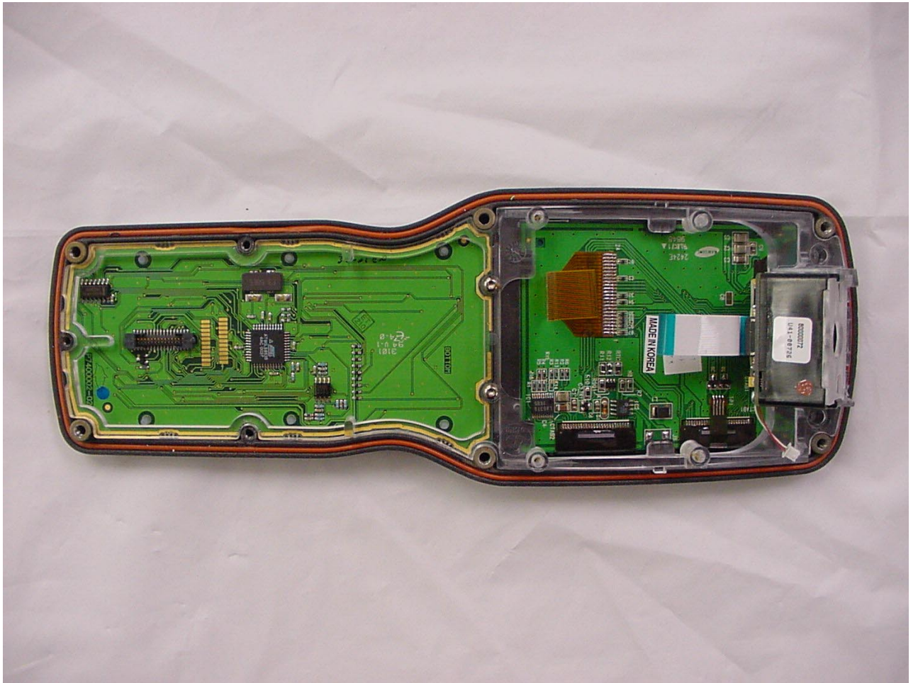
Inside View behind LCD
