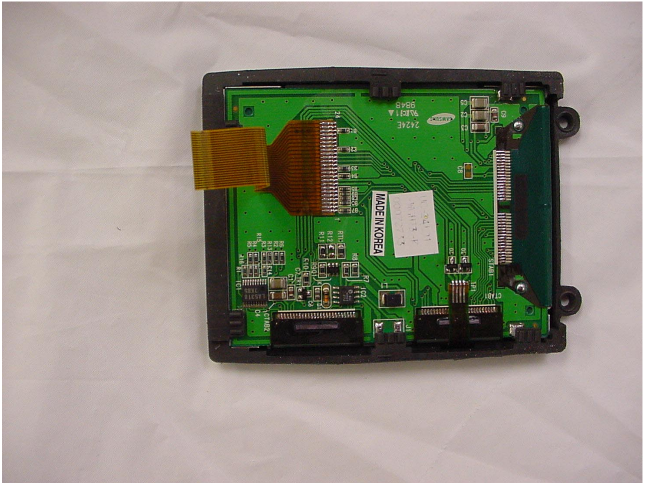
Inside View of LCD Board
