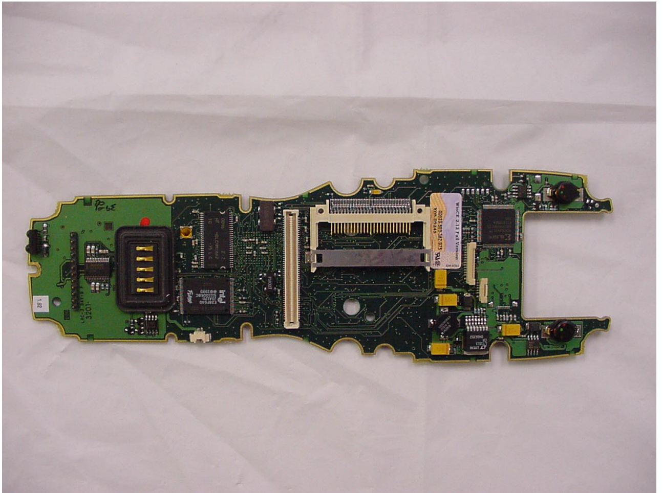
Bottom View of Motherboard
