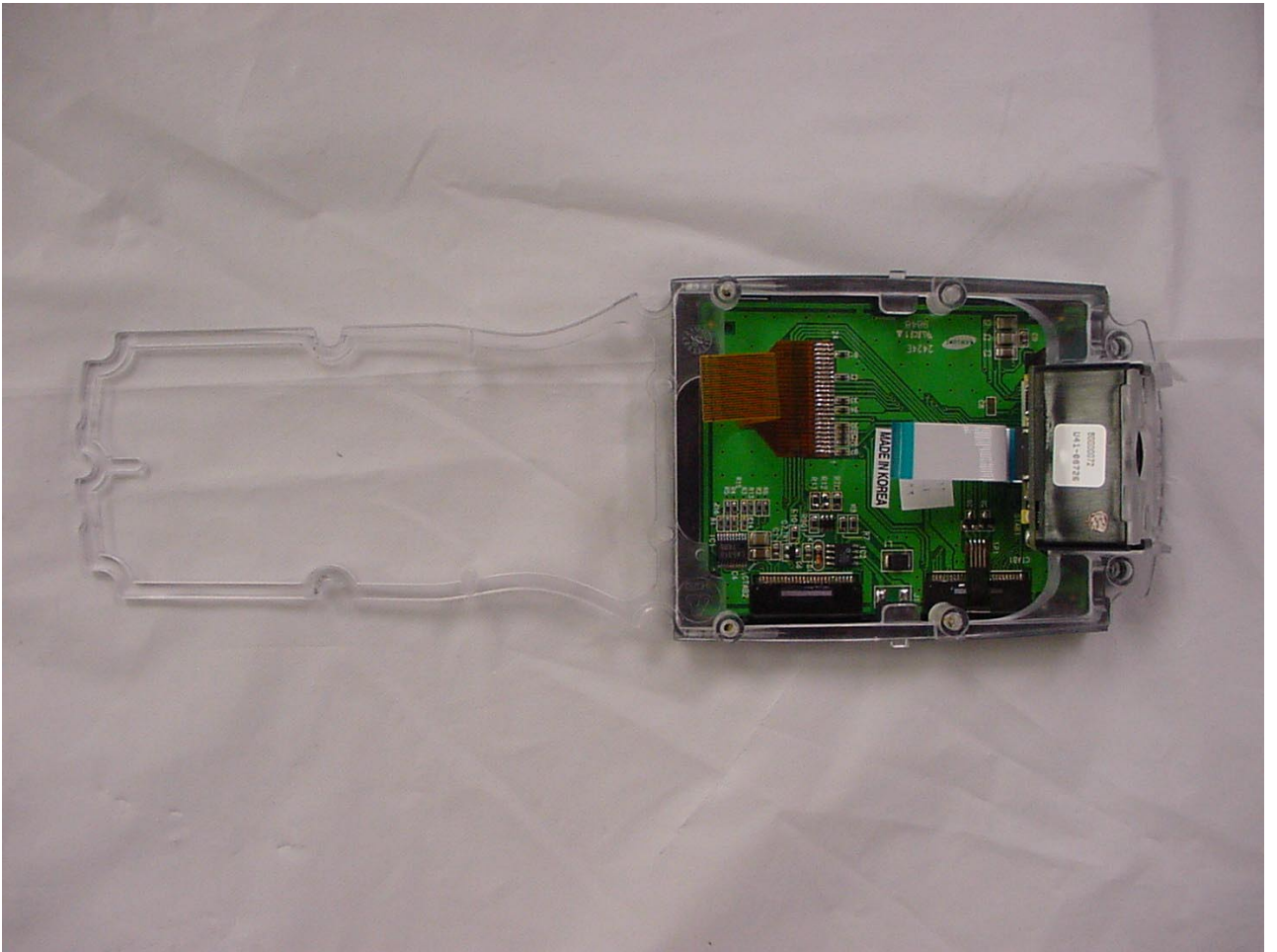
Inside View of LCD Board with Scanner
