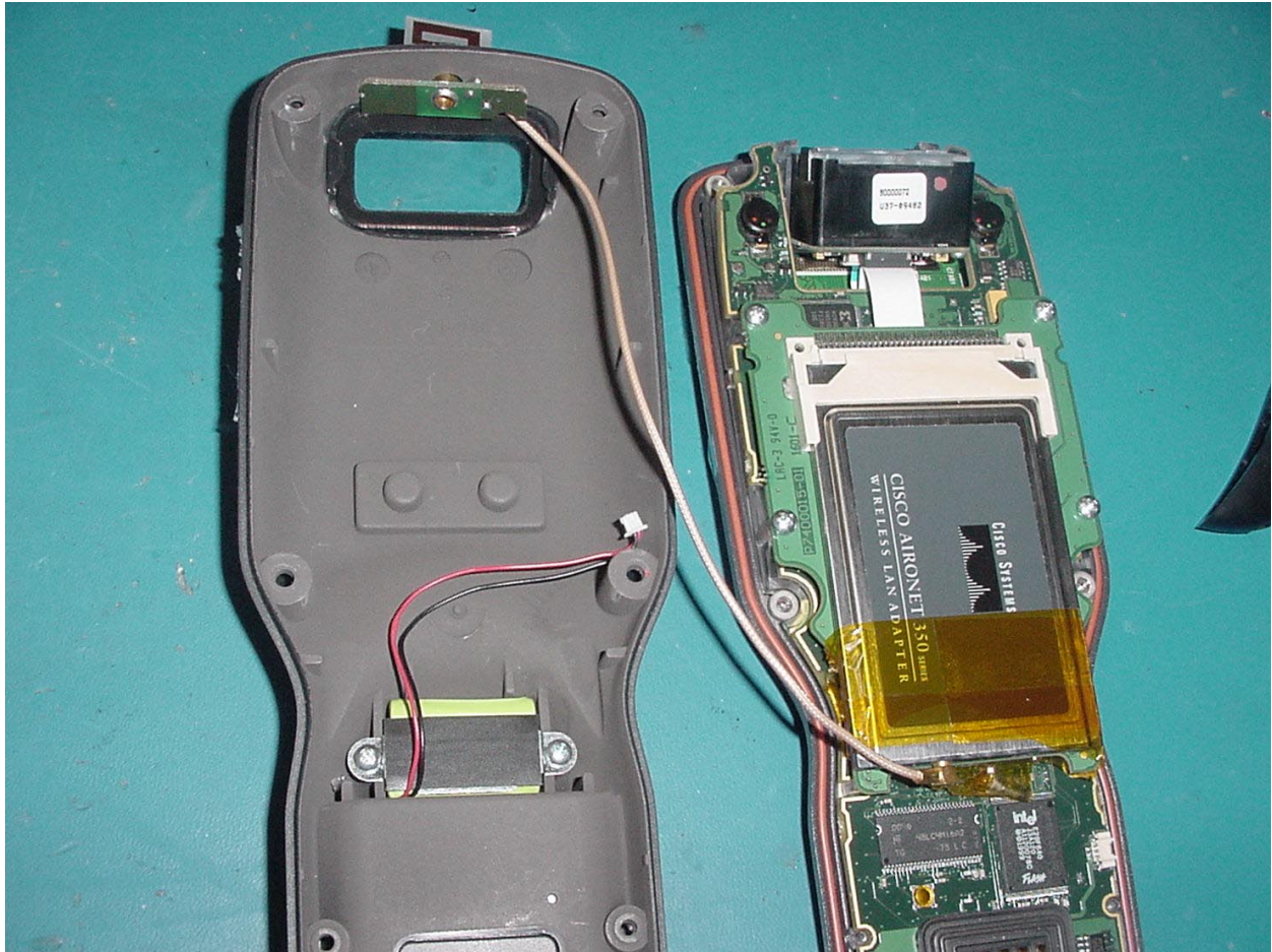
PHOTOGRAPH 6: ANTENNA CONNECTION
