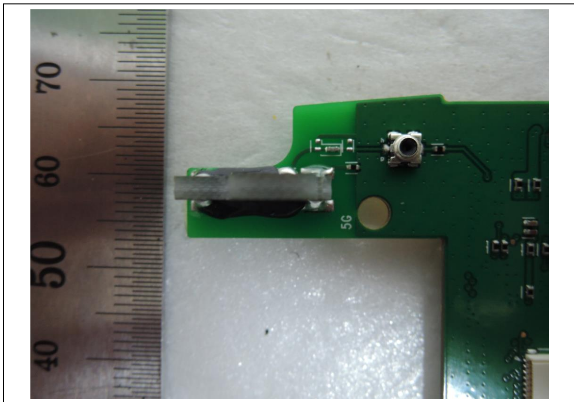
<5G WLAN Antenna>
