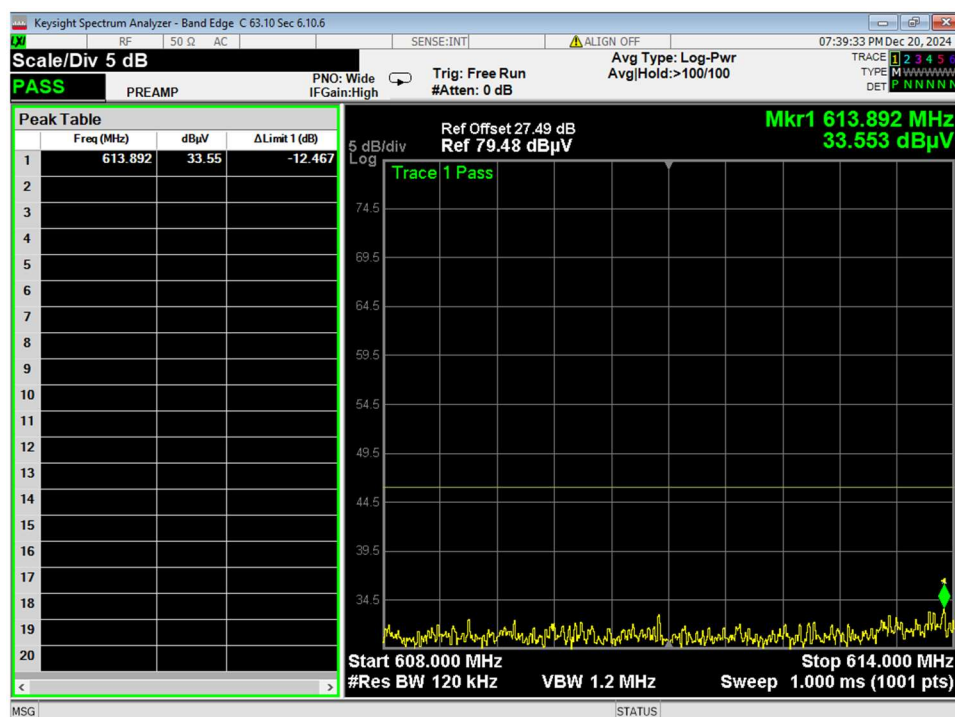
Figure 15 Bandedge Restricted Low Channel
