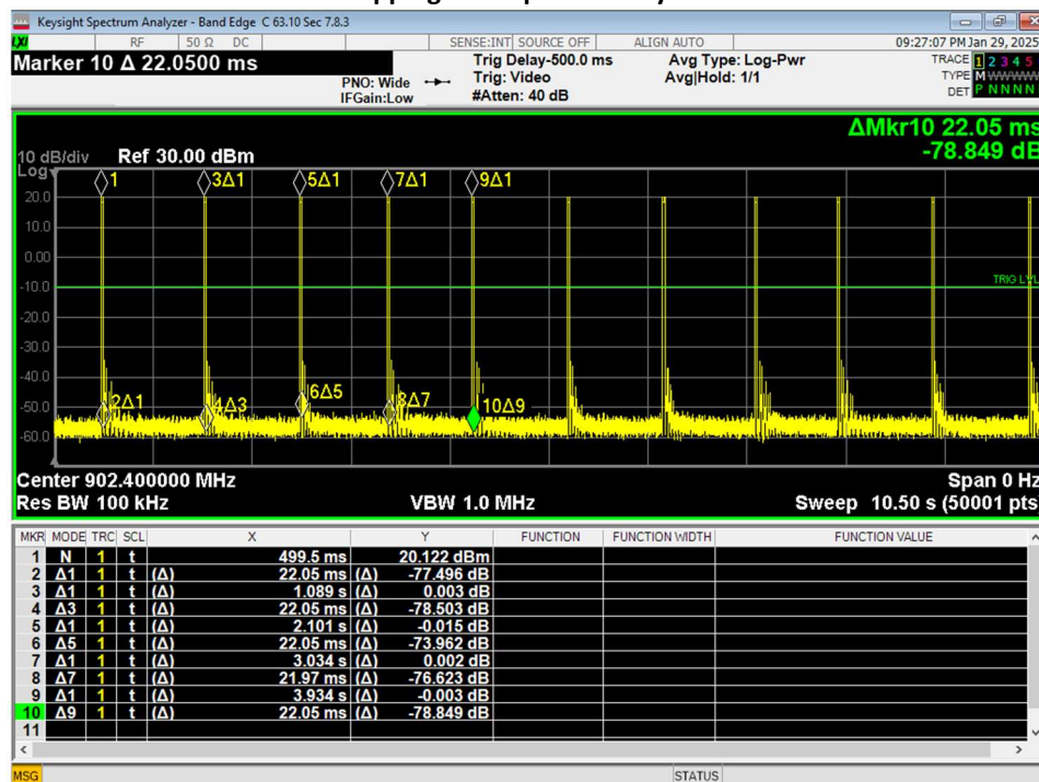
Figure 21 Channel Occupancy/ Period, Maximum of 11 Hops possible*
