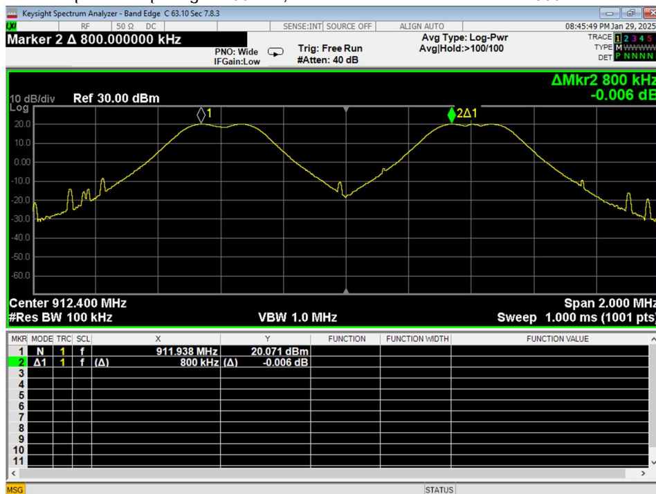
Figure 19 Minimum Frequency Separation
