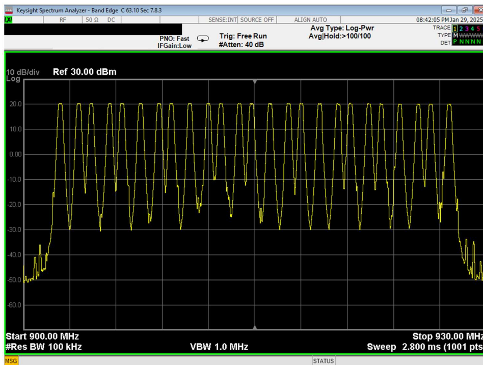
Figure 18 Hop Count, 25 Hops
