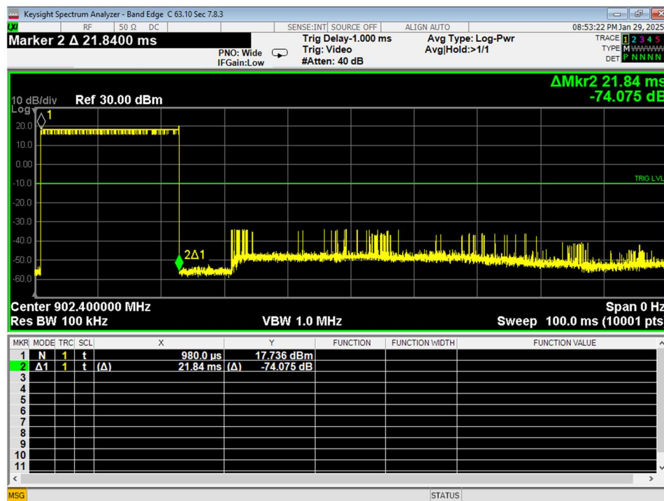
Figure 20 Channel Occupancy, On time*
