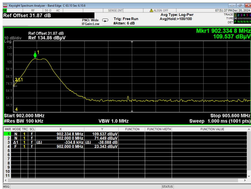
Figure 14 Bandedge Unrestricted Low Channel
