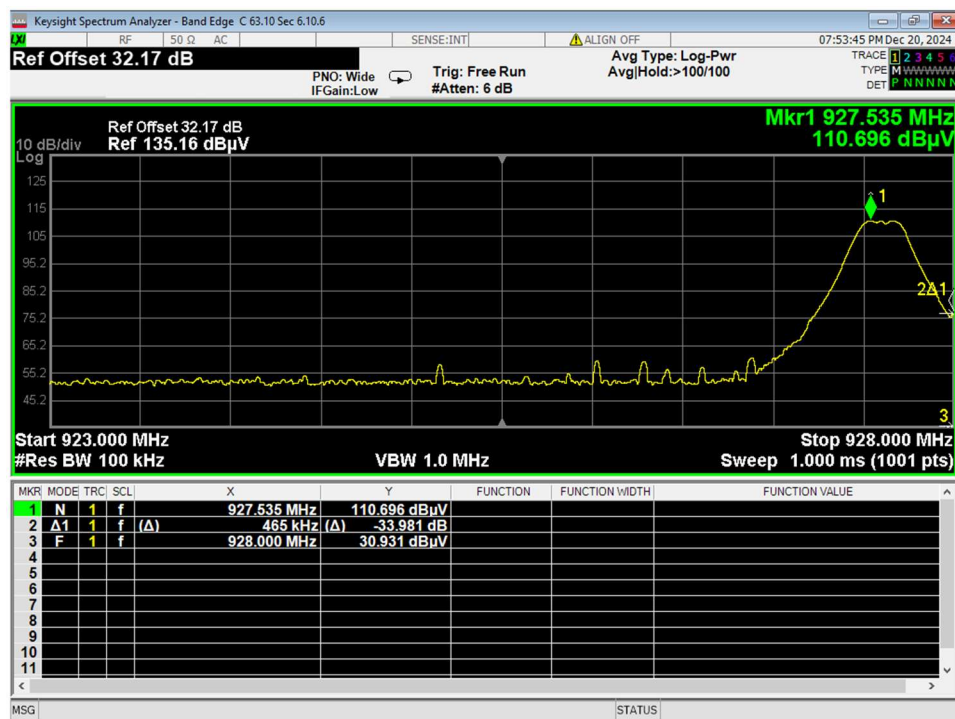
Figure 16 Bandedge Unrestricted High Channel
