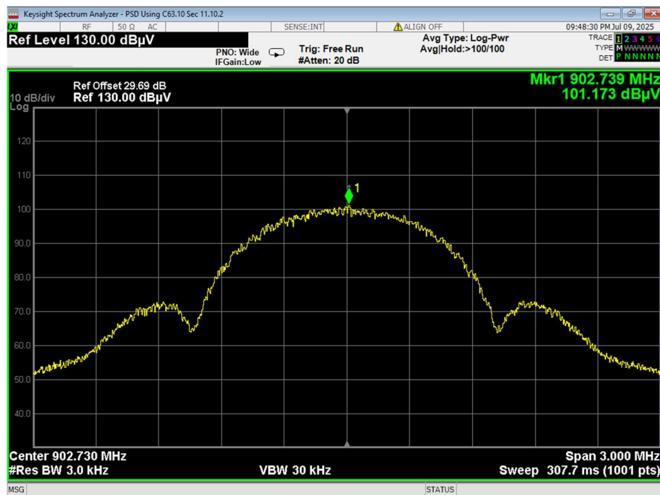
Figure 16 Power Spectral Density, Low Channel, PSD (dBm) = Field Strength (dBuV/m) – 95.23dB
