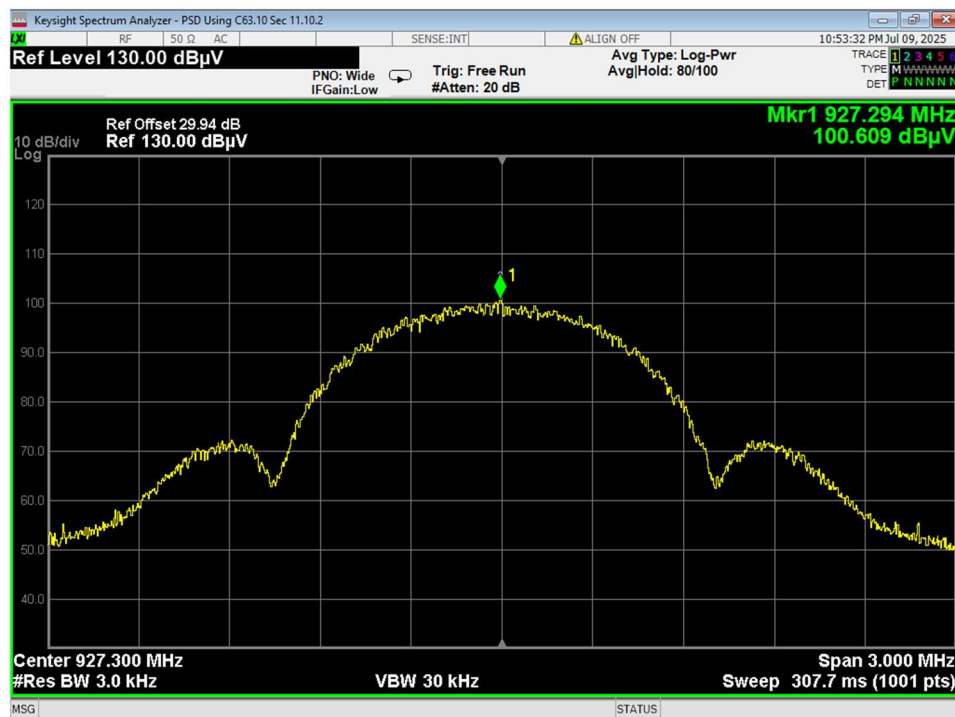
Figure 18 Power Spectral Density, High Channel, PSD (dBm) = Field Strength (dBuV/m) – 95.23dB
