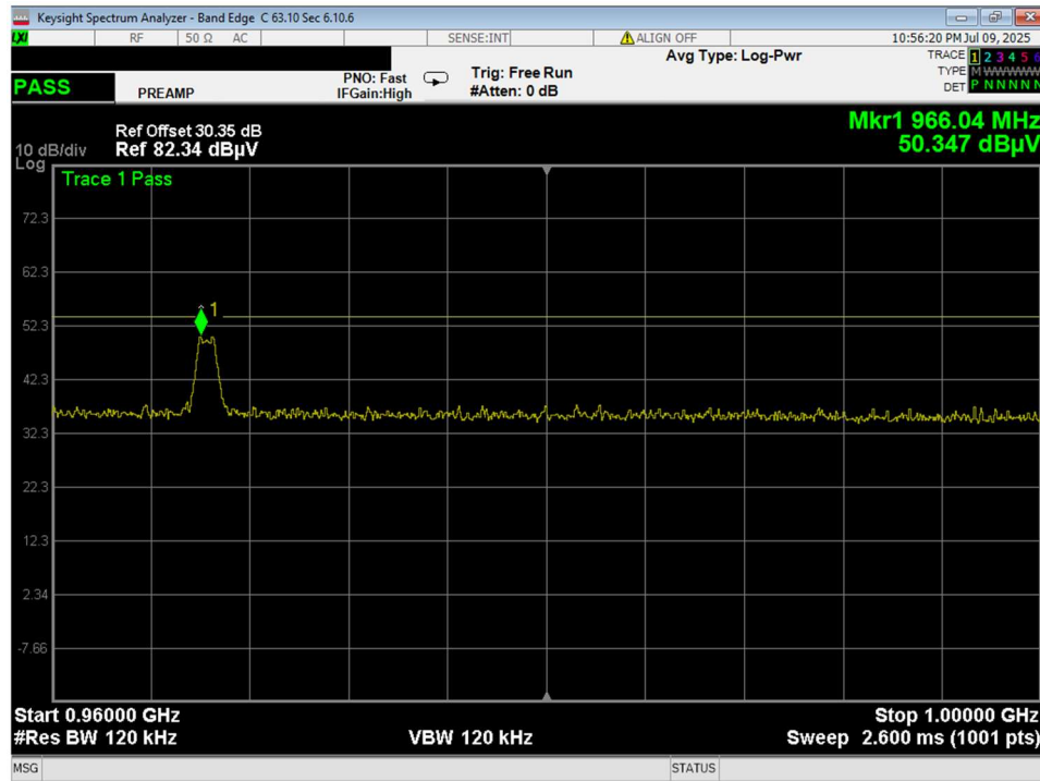
Figure 22 Bandedge Restricted High Channel.
