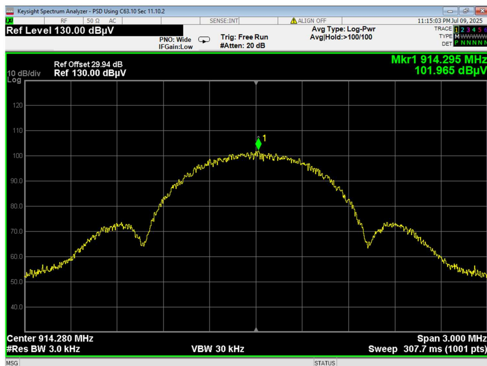
Figure 17 Power Spectral Density, Mid Channel, PSD (dBm) = Field Strength (dBuV/m) – 95.23dB
