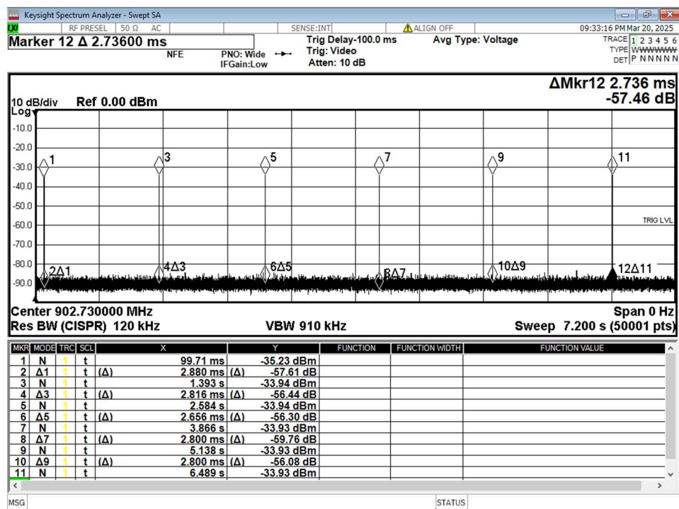
Figure 24 Channel Occupancy, On time* *Measured in hopping mode provided by the manufacturer.
