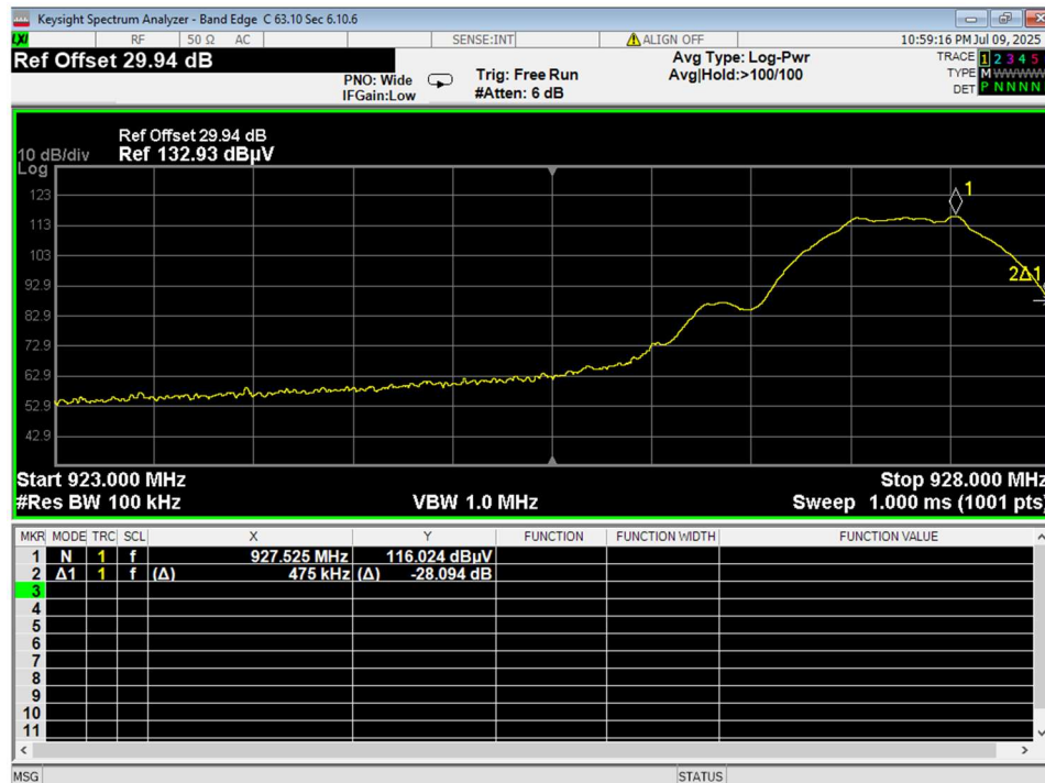
Figure 21 Bandedge Unrestricted High Channel
