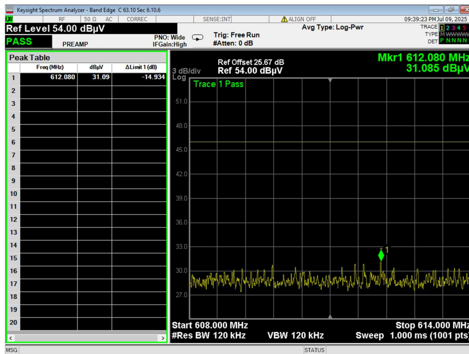
Figure 20 Bandedge Restricted Low Channel
