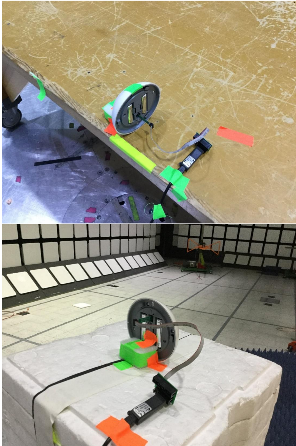
Z axis- Worst Case Orientation
