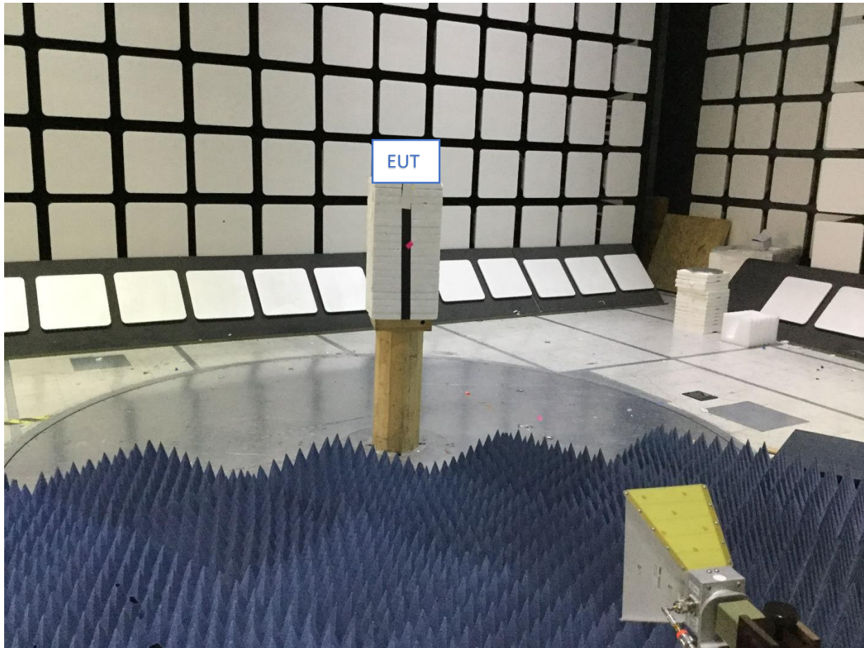
General > 1 GHz Setup
