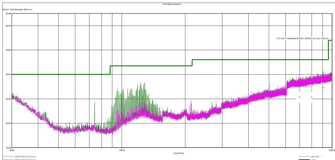
Figure 5 - Radiated Emissions Plot, Transmitter Off, 30 MHz-1GHz
