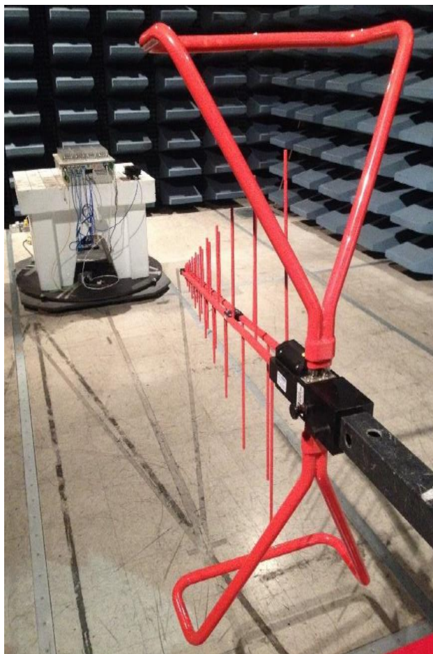
Figure 2: Radiated Emissions (Below 1GHz) Emissions Test Setup
