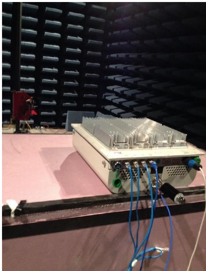
Figure 4: Radiated Emissions (Above 1GHz) Emissions Test Setup
