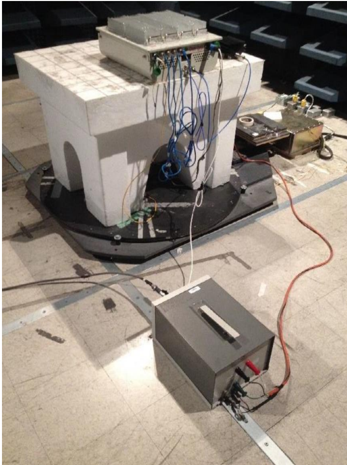
Figure 1: Conductive Emissions Test Setup
