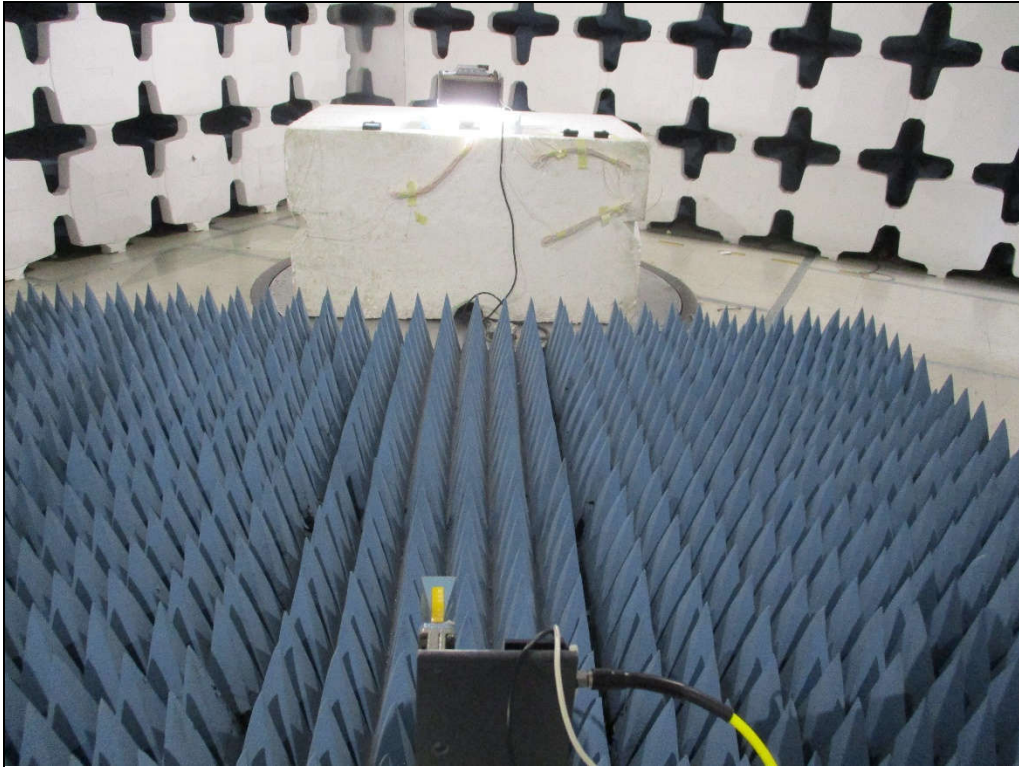
Test Setup for Radiated Emissions: 26.5GHz to 30MHz, Horizontal Polarization
